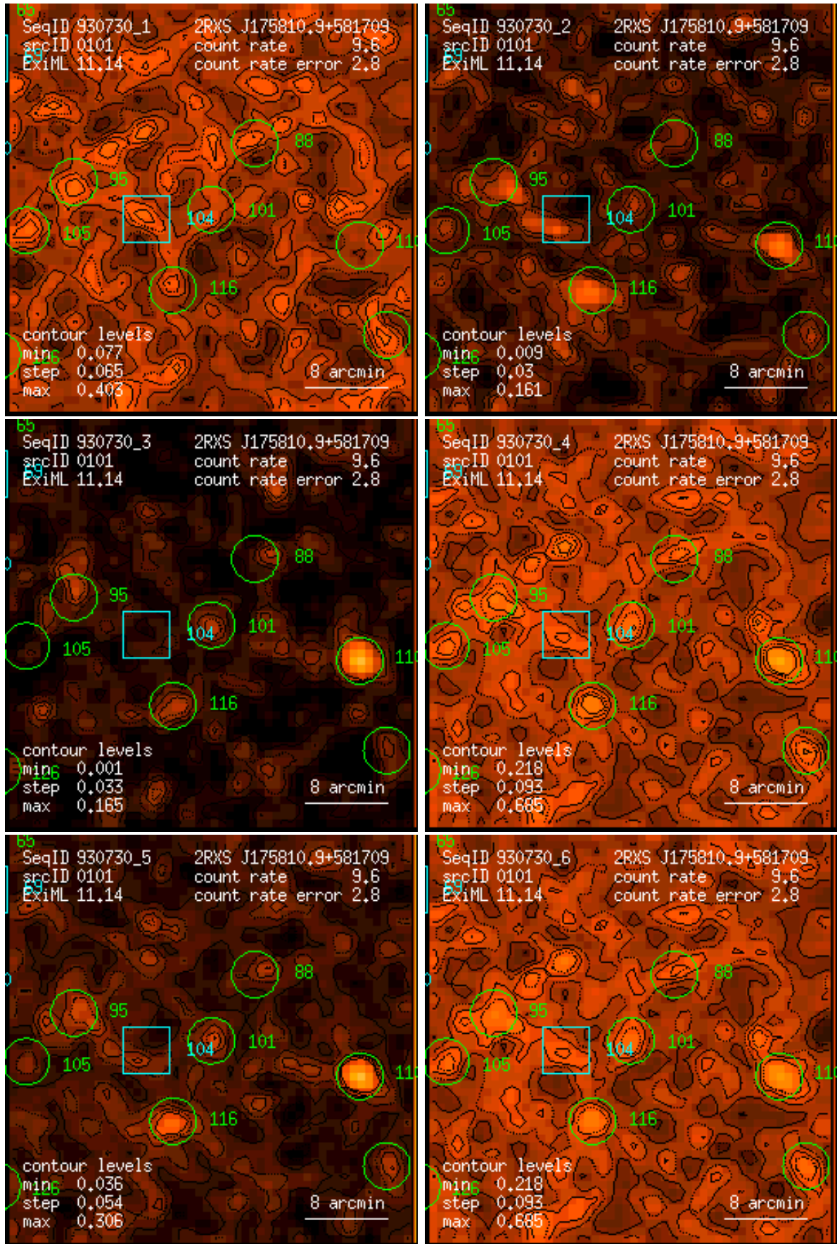
Figure 101: RASS 930730: detection 0101: band rate images, Gaussian filter: (1) PSPC channels 11 – 41, (2) 52 – 90, (3) 91 – 201, (4) 11 – 235, (5) 52 – 201, (6) 11 – 201. Broad band rates in counts/ks. Band rate contour levels in counts/ks/arcmin 2 .
