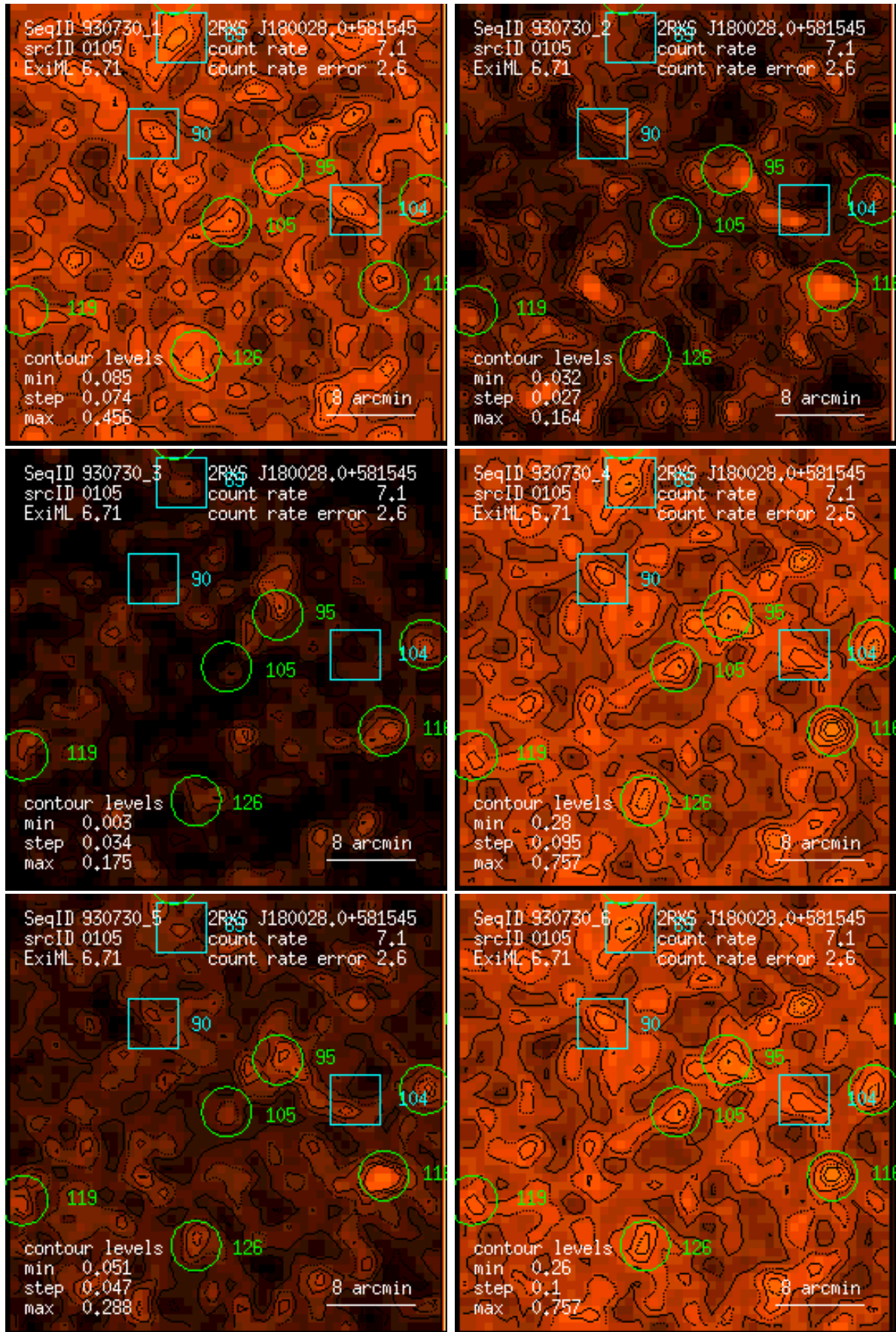
Figure 105: RASS 930730: detection 0105: band rate images, Gaussian filter: (1) PSPC channels 11 – 41, (2) 52 – 90, (3) 91 – 201, (4) 11 – 235, (5) 52 – 201, (6) 11 – 201. Broad band rates in counts/ks. Band rate contour levels in counts/ks/arcmin 2 .
