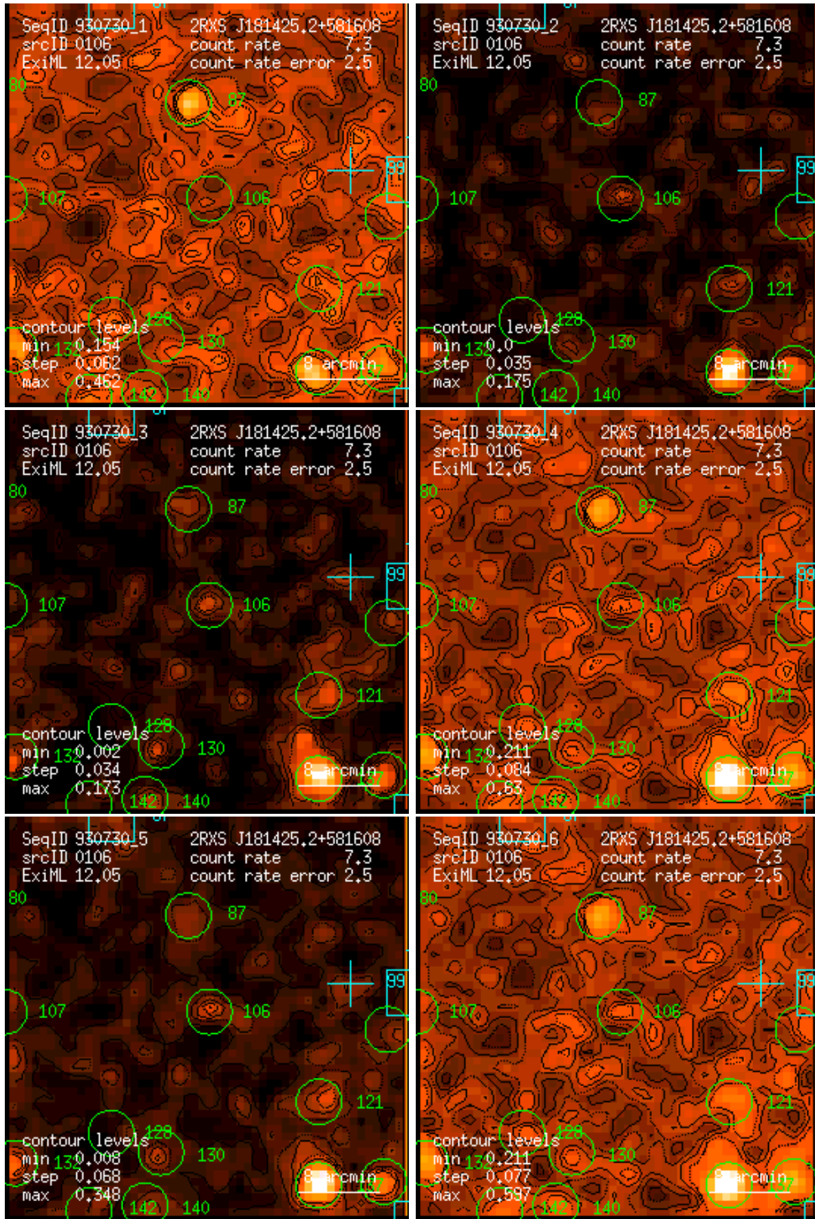
Figure 106: RASS 930730: detection 0106: band rate images, Gaussian filter: (1) PSPC channels 11 – 41, (2) 52 – 90, (3) 91 – 201, (4) 11 – 235, (5) 52 – 201, (6) 11 – 201. Broad band rates in counts/ks. Band rate contour levels in counts/ks/arcmin 2 .
