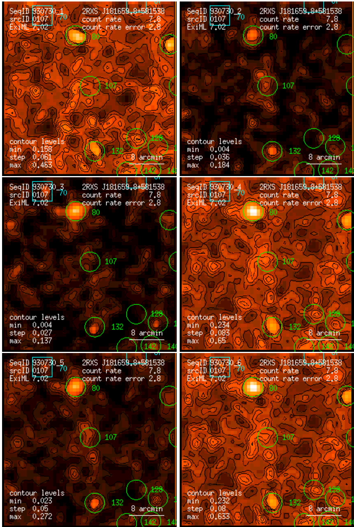
Figure 107: RASS 930730: detection 0107: band rate images, Gaussian filter: (1) PSPC channels 11 – 41, (2) 52 – 90, (3) 91 – 201, (4) 11 – 235, (5) 52 – 201, (6) 11 – 201. Broad band rates in counts/ks. Band rate contour levels in counts/ks/arcmin 2 .
