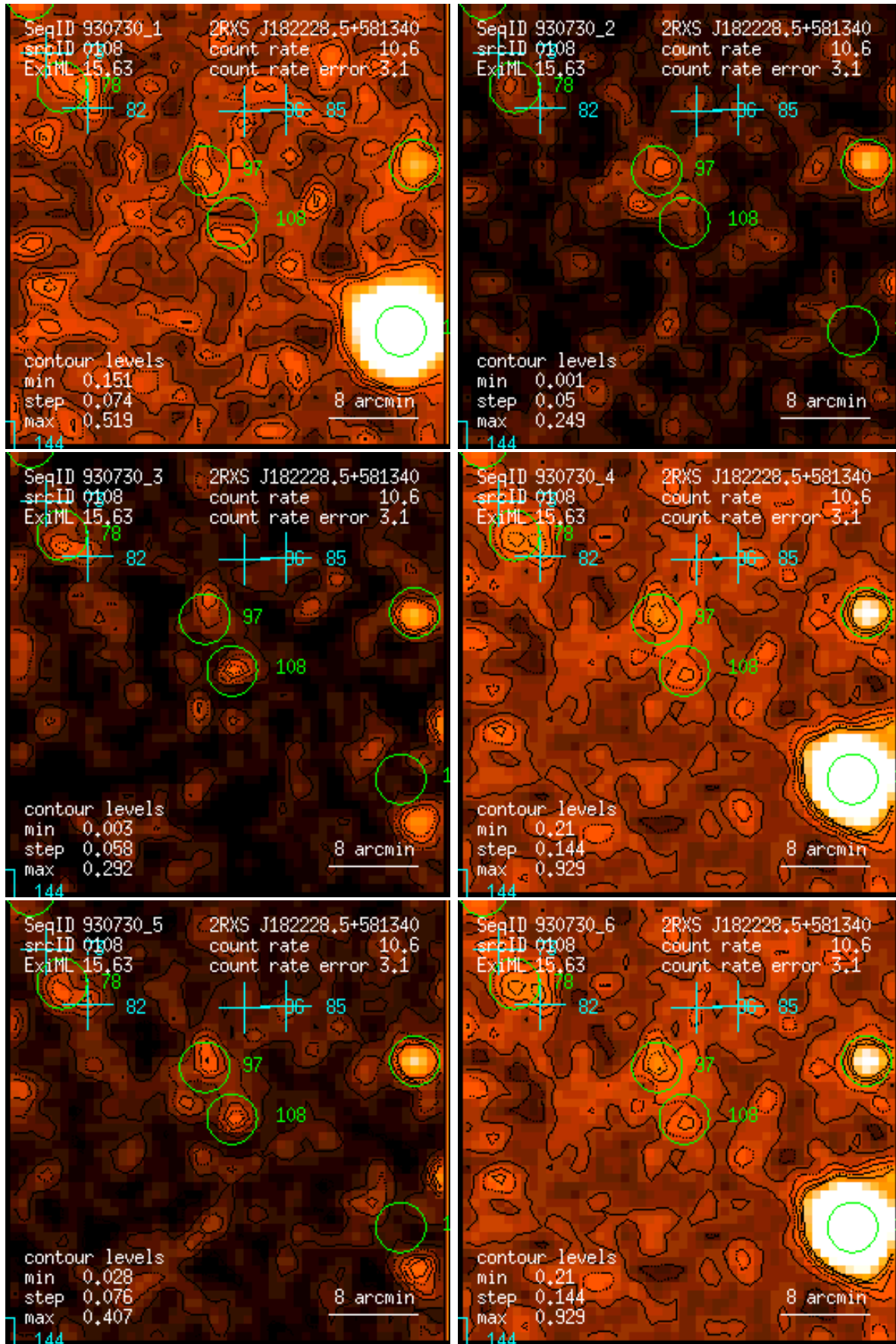
Figure 108: RASS 930730: detection 0108: band rate images, Gaussian filter: (1) PSPC channels 11 – 41, (2) 52 – 90, (3) 91 – 201, (4) 11 – 235, (5) 52 – 201, (6) 11 – 201. Broad band rates in counts/ks. Band rate contour levels in counts/ks/arcmin 2 .
