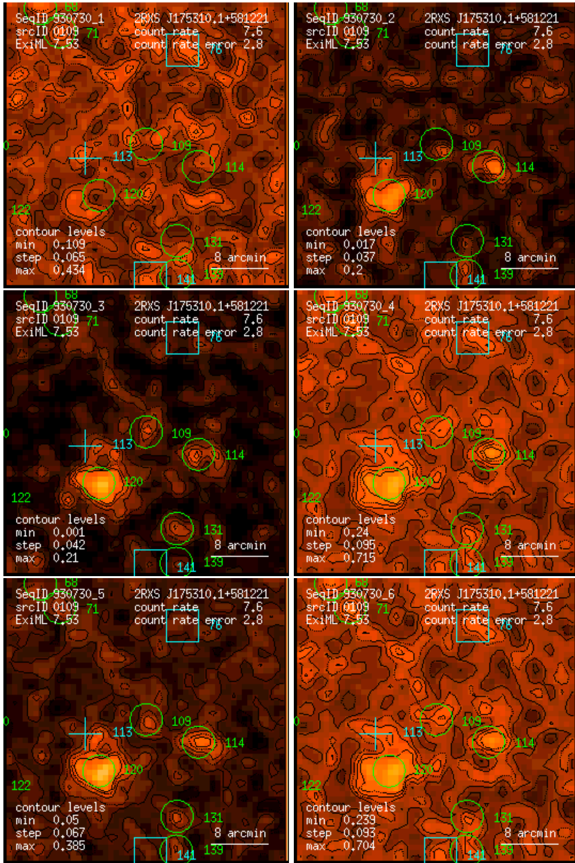
Figure 109: RASS 930730: detection 0109: band rate images, Gaussian filter: (1) PSPC channels 11 – 41, (2) 52 – 90, (3) 91 – 201, (4) 11 – 235, (5) 52 – 201, (6) 11 – 201. Broad band rates in counts/ks. Band rate contour levels in counts/ks/arcmin 2 .
