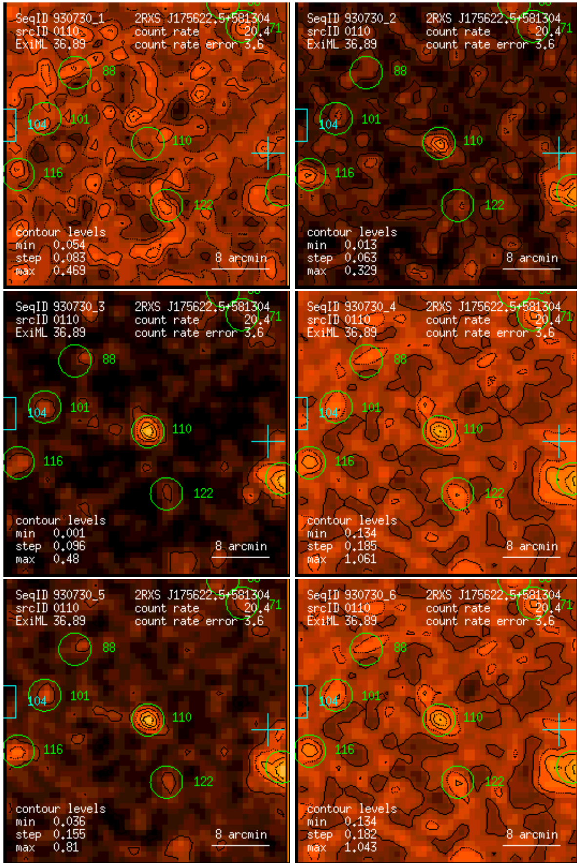
Figure 110: RASS 930730: detection 0110: band rate images, Gaussian filter: (1) PSPC channels 11 – 41, (2) 52 – 90, (3) 91 – 201, (4) 11 – 235, (5) 52 – 201, (6) 11 – 201. Broad band rates in counts/ks. Band rate contour levels in counts/ks/arcmin 2 .
