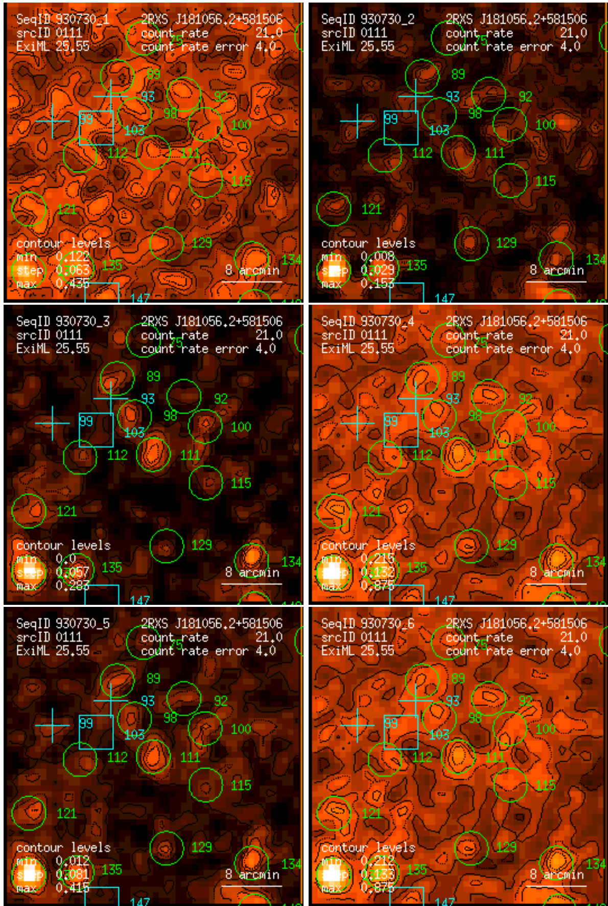
Figure 111: RASS 930730: detection 0111: band rate images, Gaussian filter: (1) PSPC channels 11 – 41, (2) 52 – 90, (3) 91 – 201, (4) 11 – 235, (5) 52 – 201, (6) 11 – 201. Broad band rates in counts/ks. Band rate contour levels in counts/ks/arcmin 2 .
