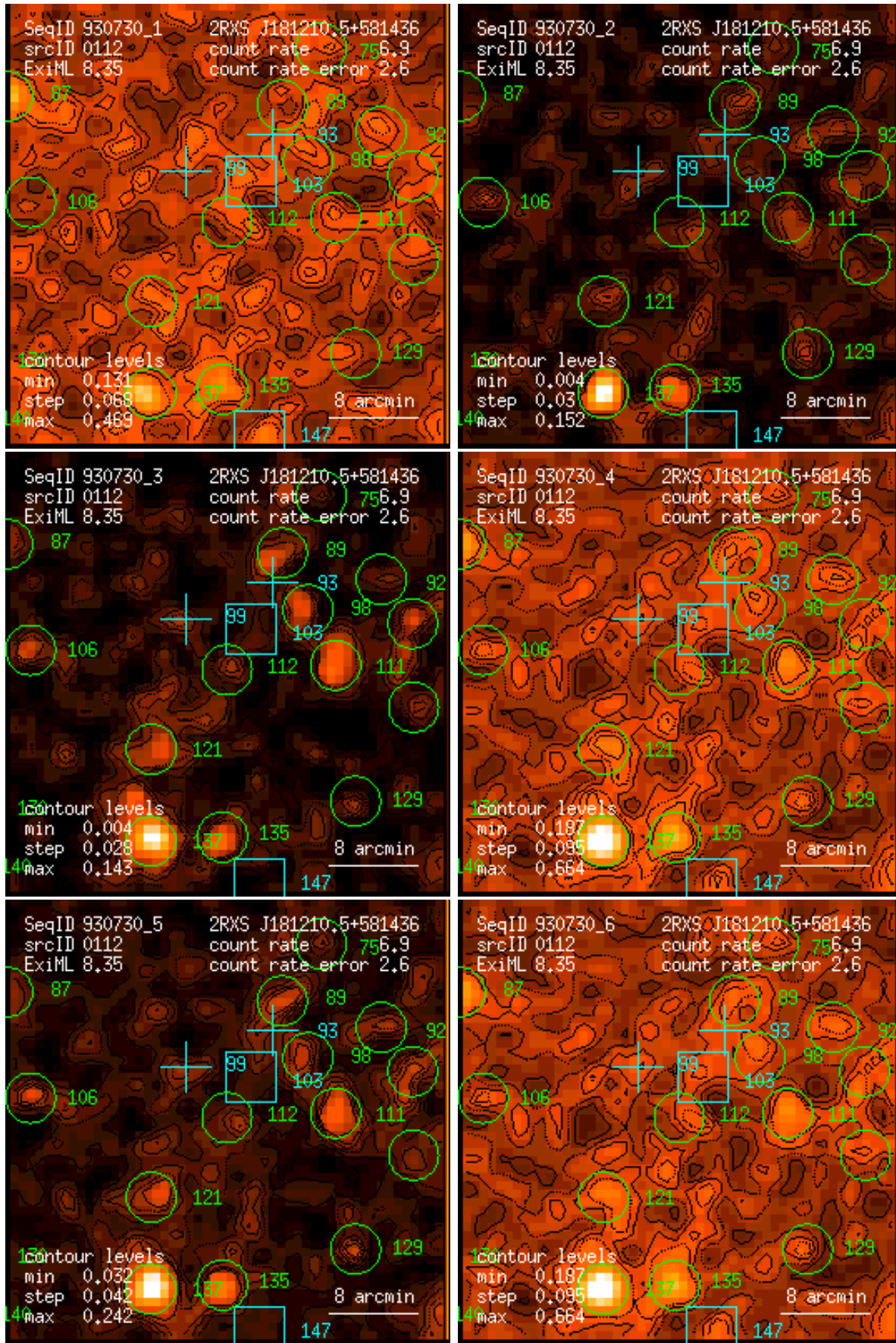
Figure 112: RASS 930730: detection 0112: band rate images, Gaussian filter: (1) PSPC channels 11 – 41, (2) 52 – 90, (3) 91 – 201, (4) 11 – 235, (5) 52 – 201, (6) 11 – 201. Broad band rates in counts/ks. Band rate contour levels in counts/ks/arcmin 2 .
