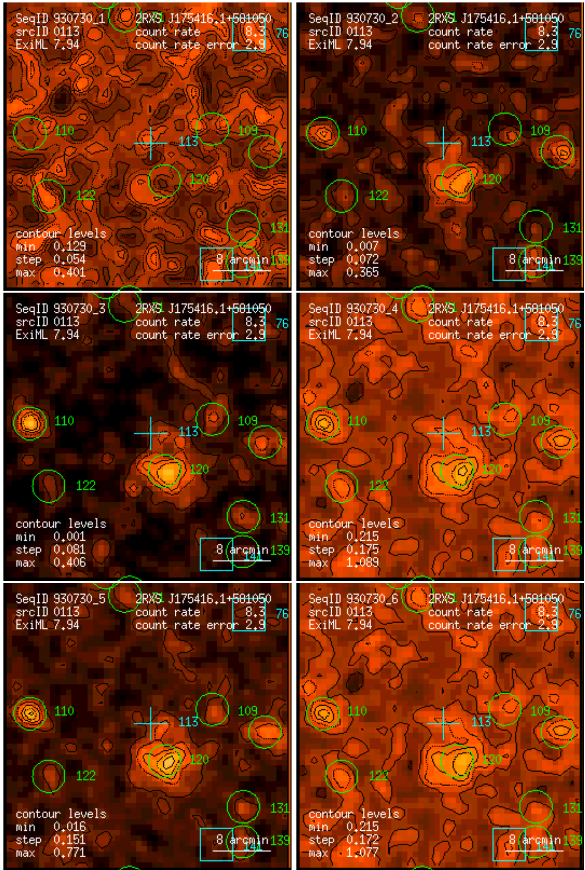
Figure 113: RASS 930730: detection 0113: band rate images, Gaussian filter: (1) PSPC channels 11 – 41, (2) 52 – 90, (3) 91 – 201, (4) 11 – 235, (5) 52 – 201, (6) 11 – 201. Broad band rates in counts/ks. Band rate contour levels in counts/ks/arcmin 2 .
