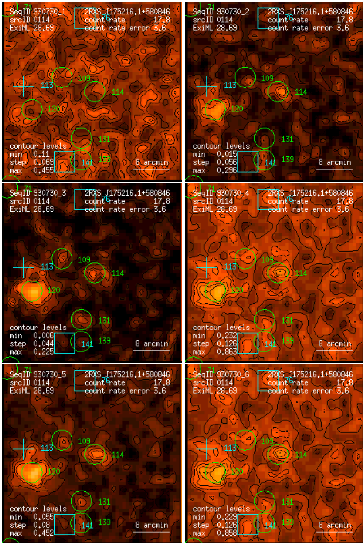
Figure 114: RASS 930730: detection 0114: band rate images, Gaussian filter: (1) PSPC channels 11 – 41, (2) 52 – 90, (3) 91 – 201, (4) 11 – 235, (5) 52 – 201, (6) 11 – 201. Broad band rates in counts/ks. Band rate contour levels in counts/ks/arcmin 2 .
