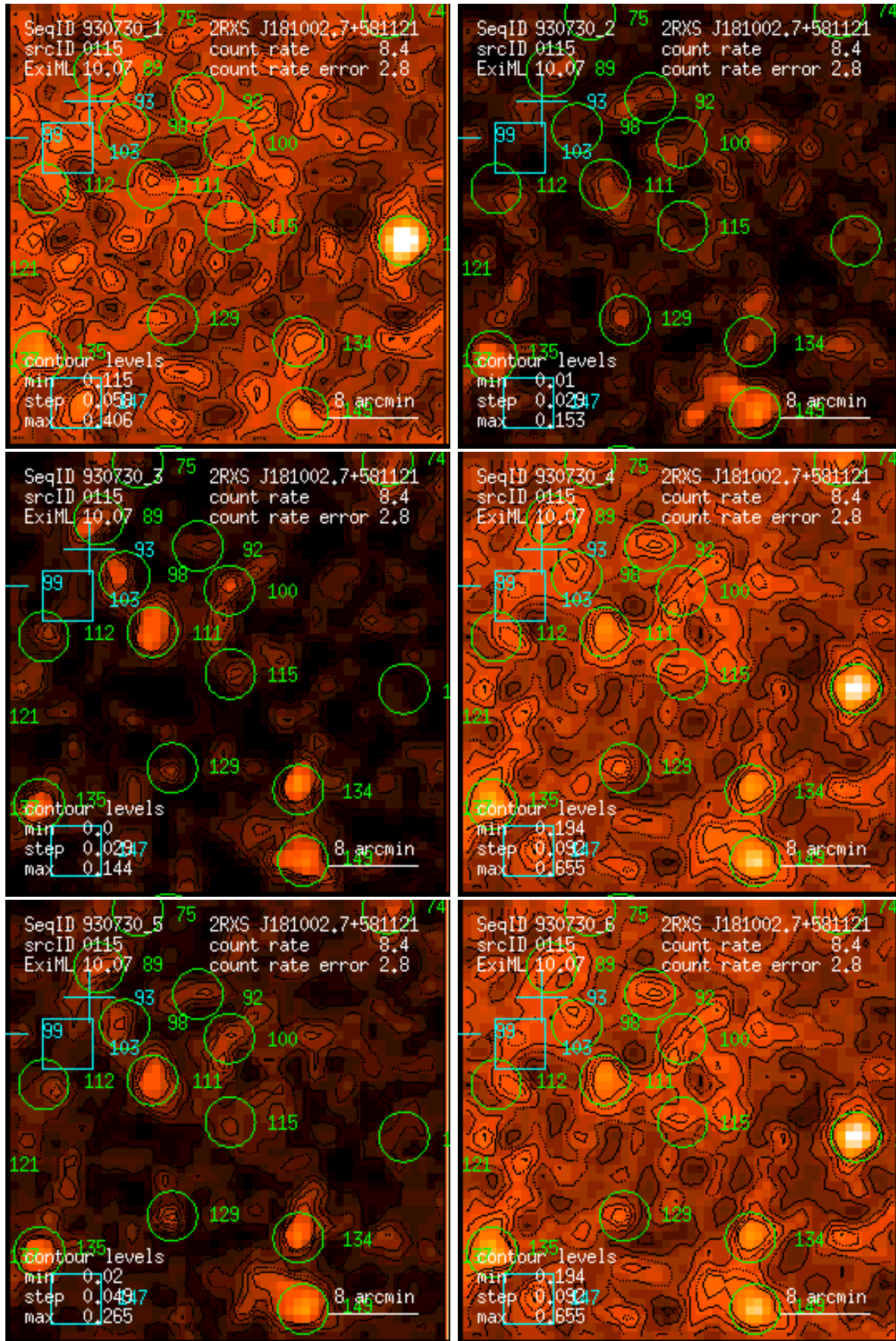
Figure 115: RASS 930730: detection 0115: band rate images, Gaussian filter: (1) PSPC channels 11 – 41, (2) 52 – 90, (3) 91 – 201, (4) 11 – 235, (5) 52 – 201, (6) 11 – 201. Broad band rates in counts/ks. Band rate contour levels in counts/ks/arcmin 2 .
