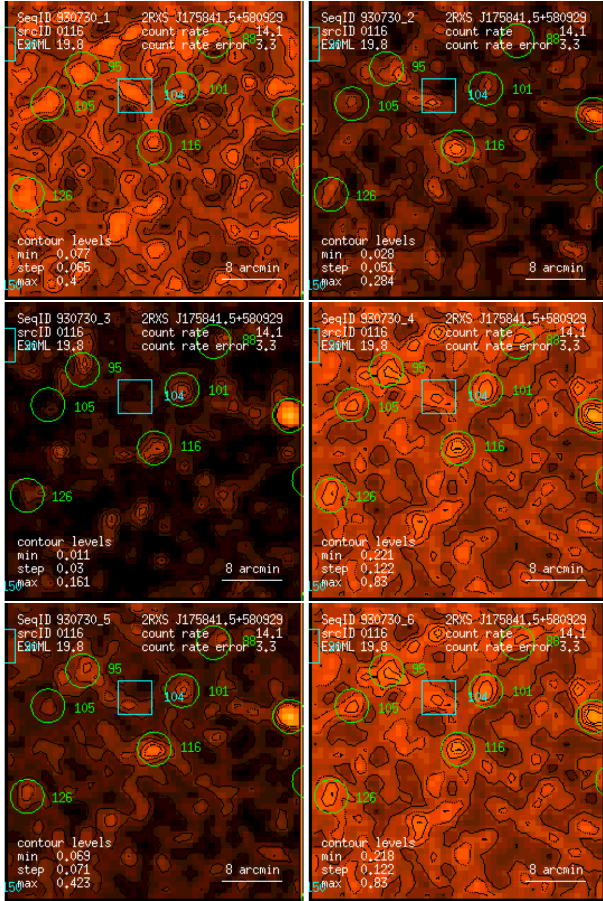
Figure 116: RASS 930730: detection 0116: band rate images, Gaussian filter: (1) PSPC channels 11 – 41, (2) 52 – 90, (3) 91 – 201, (4) 11 – 235, (5) 52 – 201, (6) 11 – 201. Broad band rates in counts/ks. Band rate contour levels in counts/ks/arcmin 2 .
