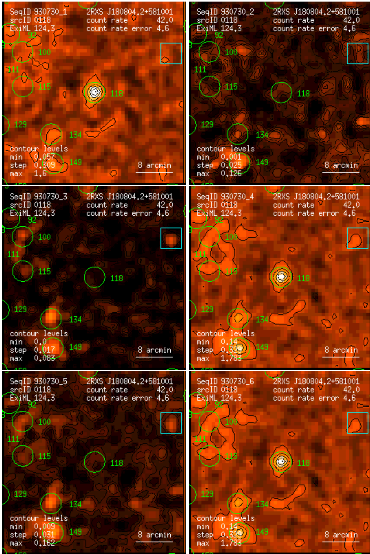
Figure 118: RASS 930730: detection 0118: band rate images, Gaussian filter: (1) PSPC channels 11 – 41, (2) 52 – 90, (3) 91 – 201, (4) 11 – 235, (5) 52 – 201, (6) 11 – 201. Broad band rates in counts/ks. Band rate contour levels in counts/ks/arcmin 2 .
