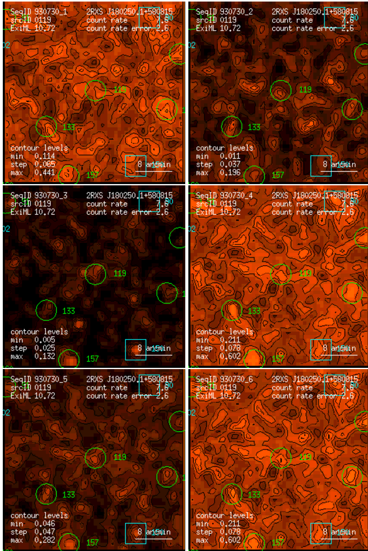
Figure 119: RASS 930730: detection 0119: band rate images, Gaussian filter: (1) PSPC channels 11 – 41, (2) 52 – 90, (3) 91 – 201, (4) 11 – 235, (5) 52 – 201, (6) 11 – 201. Broad band rates in counts/ks. Band rate contour levels in counts/ks/arcmin 2 .
