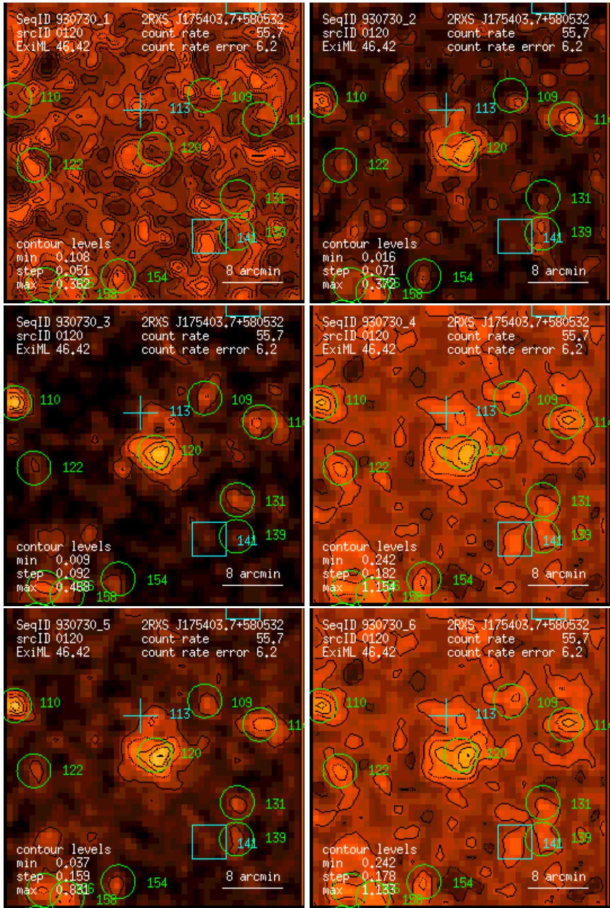
Figure 120: RASS 930730: detection 0120: band rate images, Gaussian filter: (1) PSPC channels 11 – 41, (2) 52 – 90, (3) 91 – 201, (4) 11 – 235, (5) 52 – 201, (6) 11 – 201. Broad band rates in counts/ks. Band rate contour levels in counts/ks/arcmin 2 .
