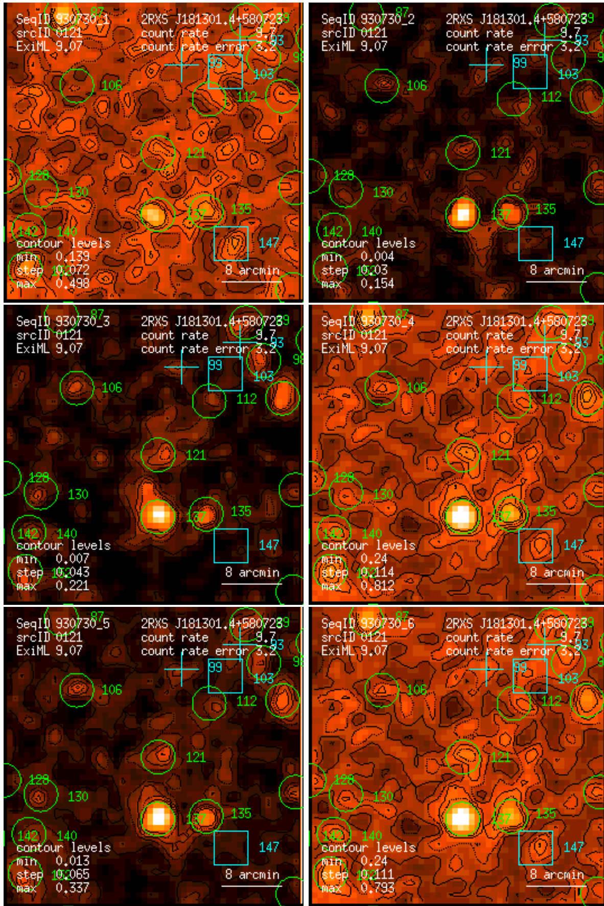
Figure 121: RASS 930730: detection 0121: band rate images, Gaussian filter: (1) PSPC channels 11 – 41, (2) 52 – 90, (3) 91 – 201, (4) 11 – 235, (5) 52 – 201, (6) 11 – 201. Broad band rates in counts/ks. Band rate contour levels in counts/ks/arcmin 2 .
