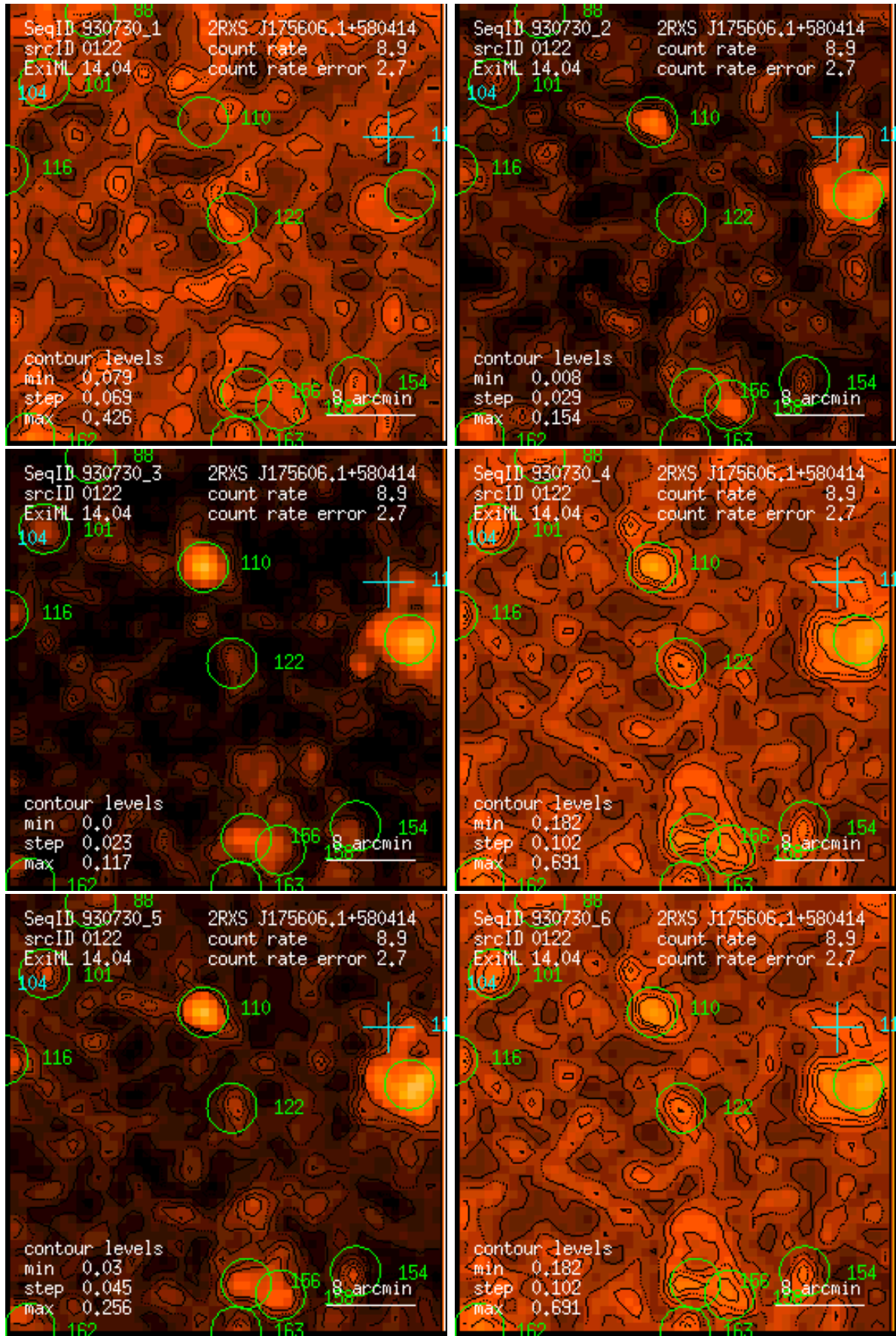
Figure 122: RASS 930730: detection 0122: band rate images, Gaussian filter: (1) PSPC channels 11 – 41, (2) 52 – 90, (3) 91 – 201, (4) 11 – 235, (5) 52 – 201, (6) 11 – 201. Broad band rates in counts/ks. Band rate contour levels in counts/ks/arcmin 2 .
