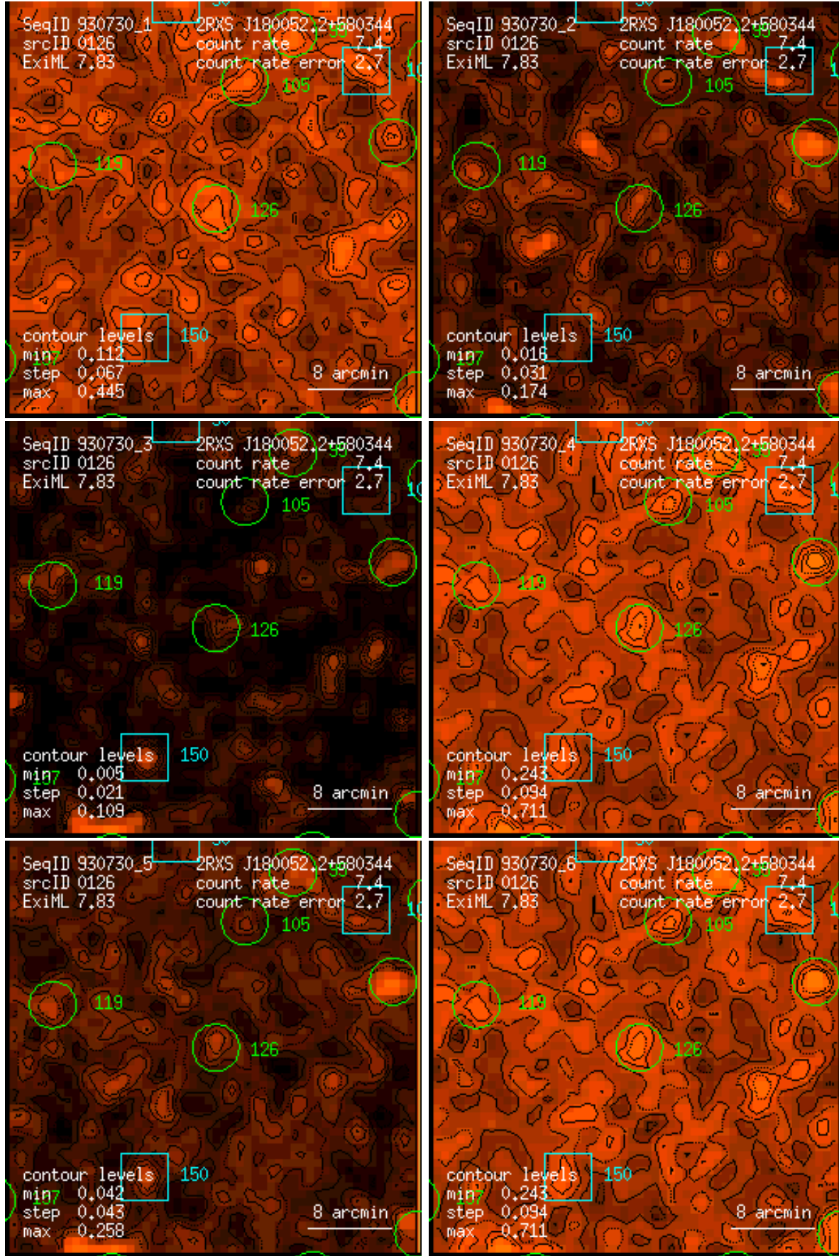
Figure 126: RASS 930730: detection 0126: band rate images, Gaussian filter: (1) PSPC channels 11 – 41, (2) 52 – 90, (3) 91 – 201, (4) 11 – 235, (5) 52 – 201, (6) 11 – 201. Broad band rates in counts/ks. Band rate contour levels in counts/ks/arcmin 2 .
