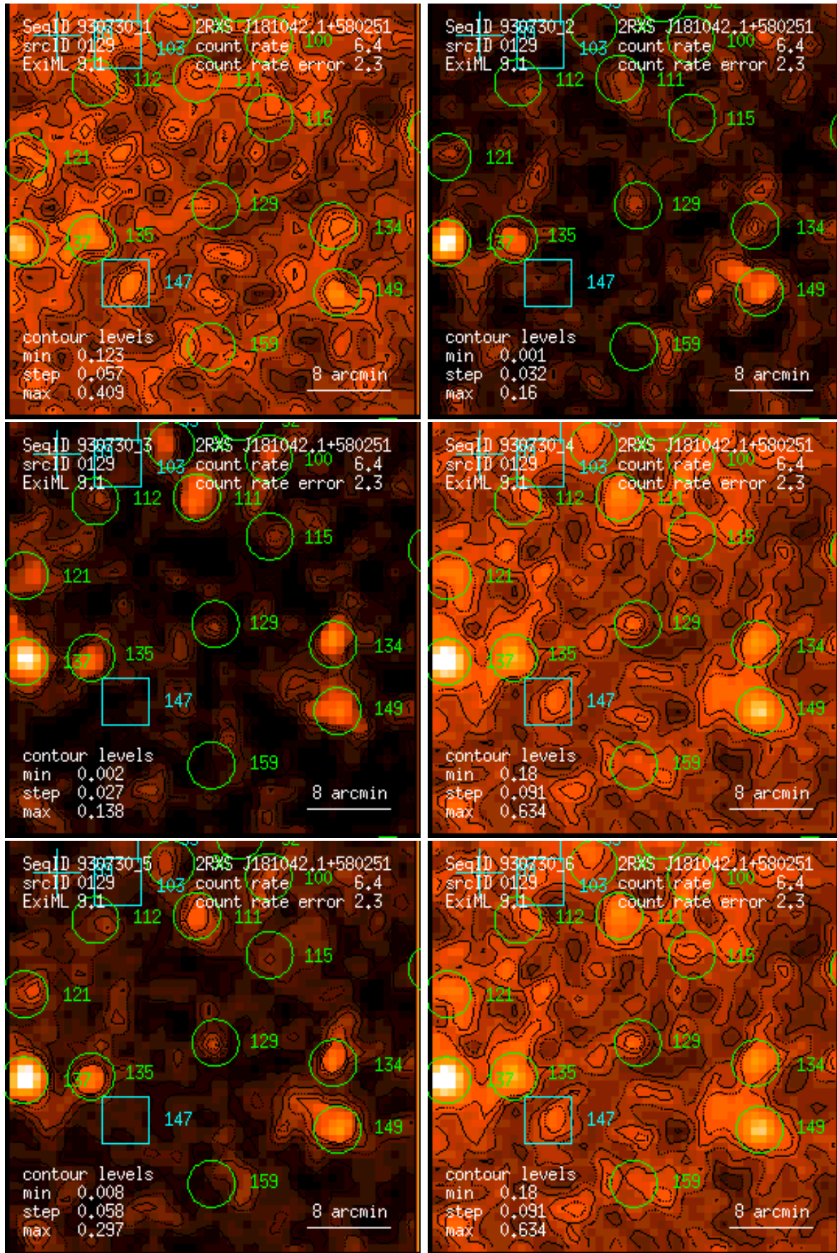
Figure 129: RASS 930730: detection 0129: band rate images, Gaussian filter: (1) PSPC channels 11 – 41, (2) 52 – 90, (3) 91 – 201, (4) 11 – 235, (5) 52 – 201, (6) 11 – 201. Broad band rates in counts/ks. Band rate contour levels in counts/ks/arcmin 2 .
