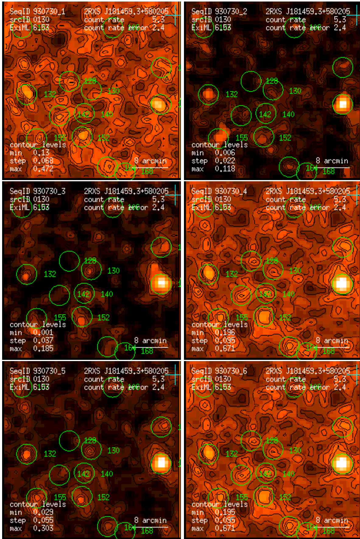
Figure 130: RASS 930730: detection 0130: band rate images, Gaussian filter: (1) PSPC channels 11 – 41, (2) 52 – 90, (3) 91 – 201, (4) 11 – 235, (5) 52 – 201, (6) 11 – 201. Broad band rates in counts/ks. Band rate contour levels in counts/ks/arcmin 2 .
