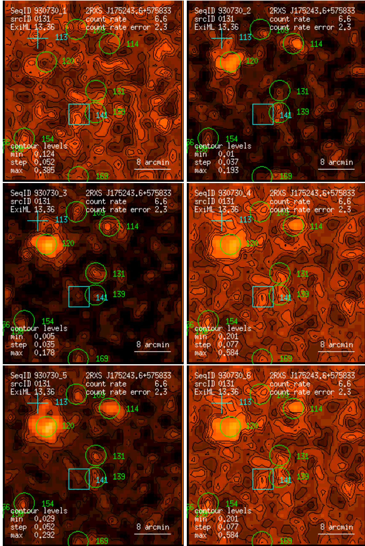
Figure 131: RASS 930730: detection 0131: band rate images, Gaussian filter: (1) PSPC channels 11 – 41, (2) 52 – 90, (3) 91 – 201, (4) 11 – 235, (5) 52 – 201, (6) 11 – 201. Broad band rates in counts/ks. Band rate contour levels in counts/ks/arcmin 2 .
