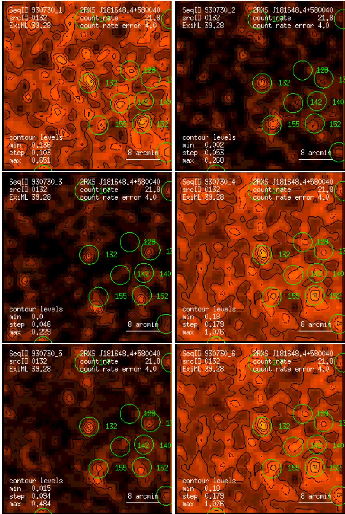
Figure 132: RASS 930730: detection 0132: band rate images, Gaussian filter: (1) PSPC channels 11 – 41, (2) 52 – 90, (3) 91 – 201, (4) 11 – 235, (5) 52 – 201, (6) 11 – 201. Broad band rates in counts/ks. Band rate contour levels in counts/ks/arcmin 2 .
