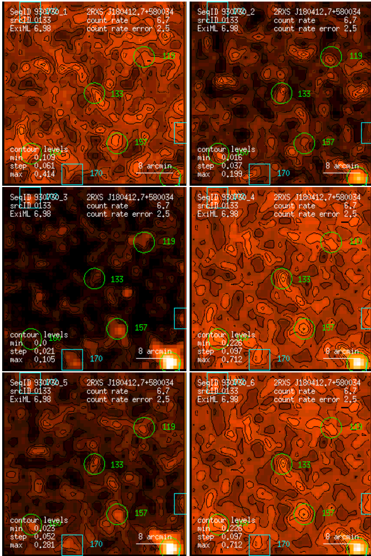
Figure 133: RASS 930730: detection 0133: band rate images, Gaussian filter: (1) PSPC channels 11 – 41, (2) 52 – 90, (3) 91 – 201, (4) 11 – 235, (5) 52 – 201, (6) 11 – 201. Broad band rates in counts/ks. Band rate contour levels in counts/ks/arcmin 2 .
