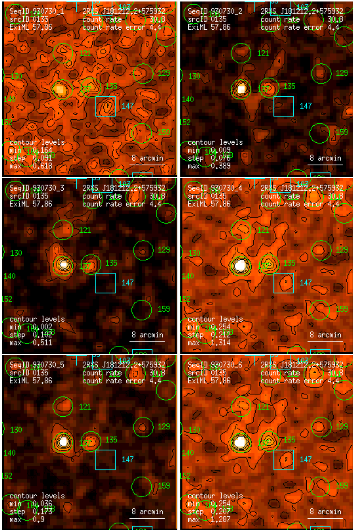
Figure 135: RASS 930730: detection 0135: band rate images, Gaussian filter: (1) PSPC channels 11 – 41, (2) 52 – 90, (3) 91 – 201, (4) 11 – 235, (5) 52 – 201, (6) 11 – 201. Broad band rates in counts/ks. Band rate contour levels in counts/ks/arcmin 2 .
