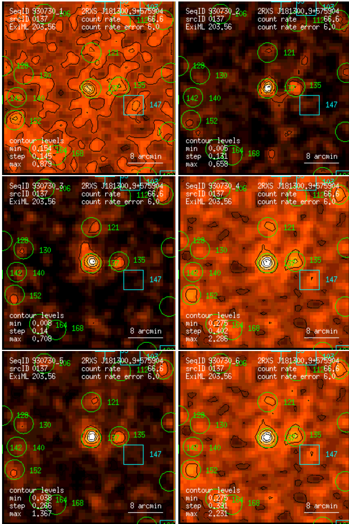
Figure 137: RASS 930730: detection 0137: band rate images, Gaussian filter: (1) PSPC channels 11 – 41, (2) 52 – 90, (3) 91 – 201, (4) 11 – 235, (5) 52 – 201, (6) 11 – 201. Broad band rates in counts/ks. Band rate contour levels in counts/ks/arcmin 2 .
