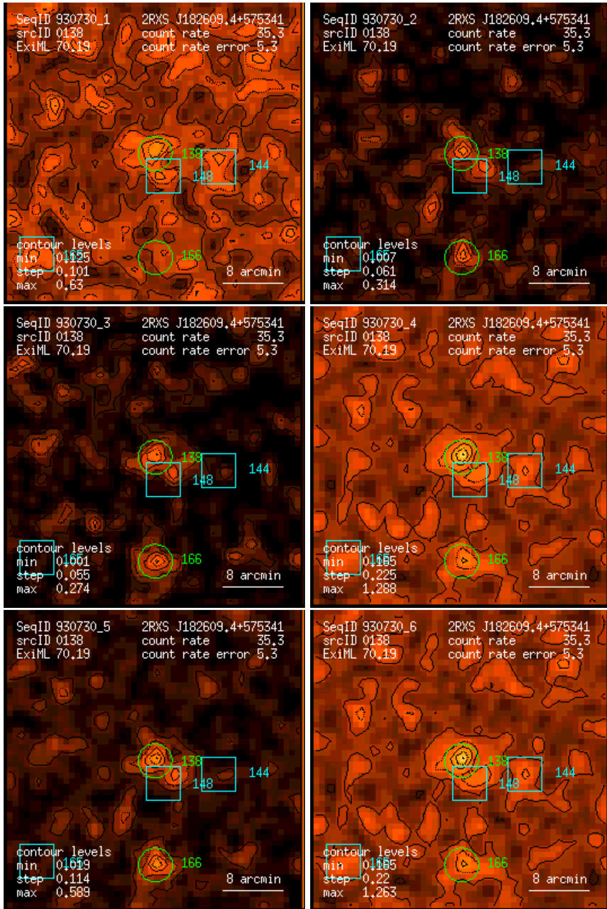
Figure 138: RASS 930730: detection 0138: band rate images, Gaussian filter: (1) PSPC channels 11 – 41, (2) 52 – 90, (3) 91 – 201, (4) 11 – 235, (5) 52 – 201, (6) 11 – 201. Broad band rates in counts/ks. Band rate contour levels in counts/ks/arcmin 2 .
