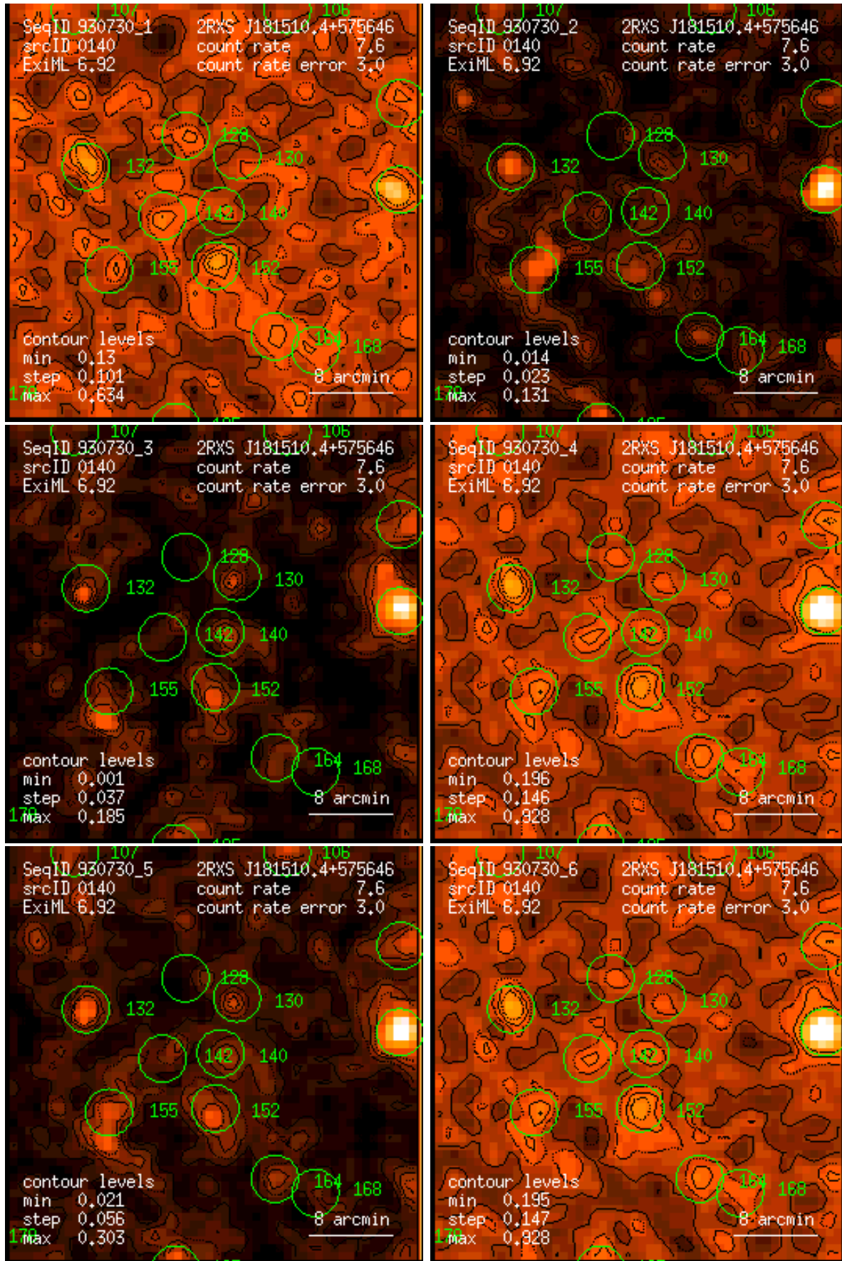
Figure 140: RASS 930730: detection 0140: band rate images, Gaussian filter: (1) PSPC channels 11 – 41, (2) 52 – 90, (3) 91 – 201, (4) 11 – 235, (5) 52 – 201, (6) 11 – 201. Broad band rates in counts/ks. Band rate contour levels in counts/ks/arcmin 2 .
