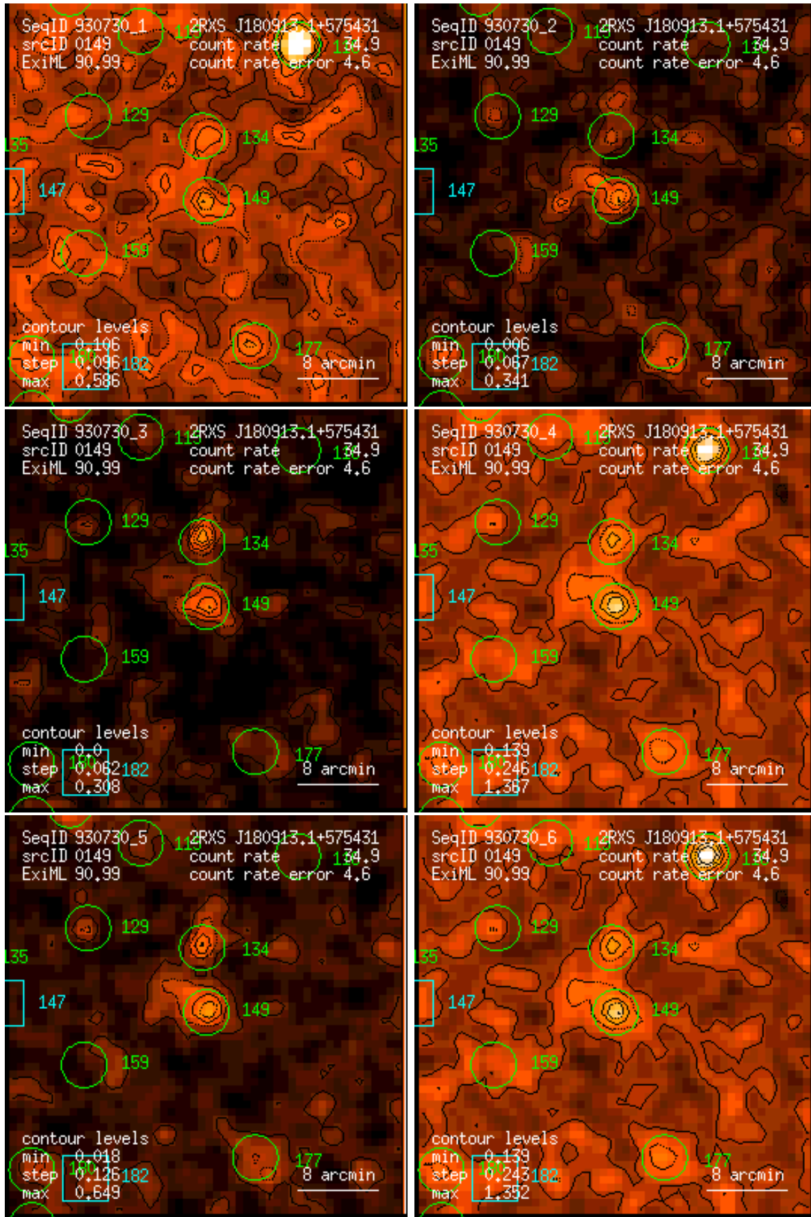
Figure 149: RASS 930730: detection 0149: band rate images, Gaussian filter: (1) PSPC channels 11 – 41, (2) 52 – 90, (3) 91 – 201, (4) 11 – 235, (5) 52 – 201, (6) 11 – 201. Broad band rates in counts/ks. Band rate contour levels in counts/ks/arcmin 2 .
