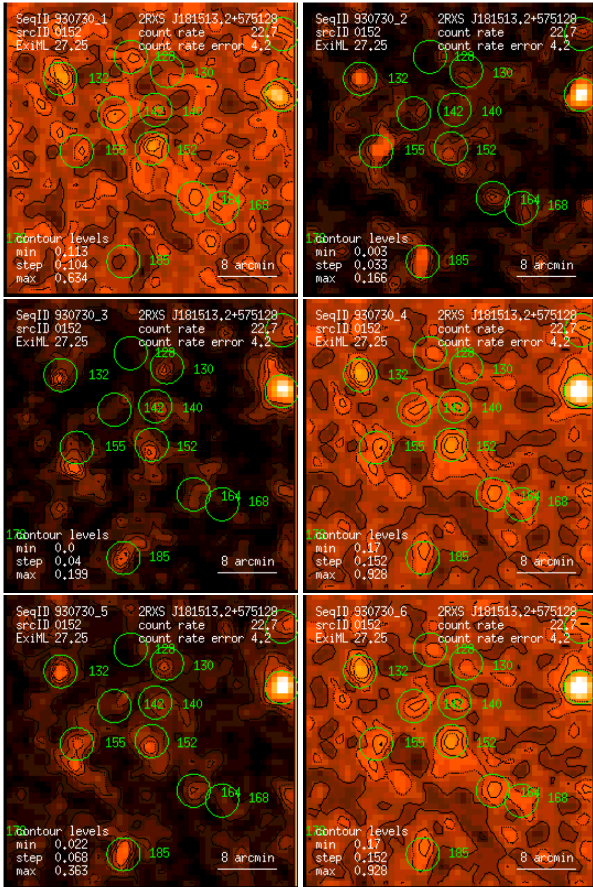
Figure 152: RASS 930730: detection 0152: band rate images, Gaussian filter: (1) PSPC channels 11 – 41, (2) 52 – 90, (3) 91 – 201, (4) 11 – 235, (5) 52 – 201, (6) 11 – 201. Broad band rates in counts/ks. Band rate contour levels in counts/ks/arcmin 2 .
