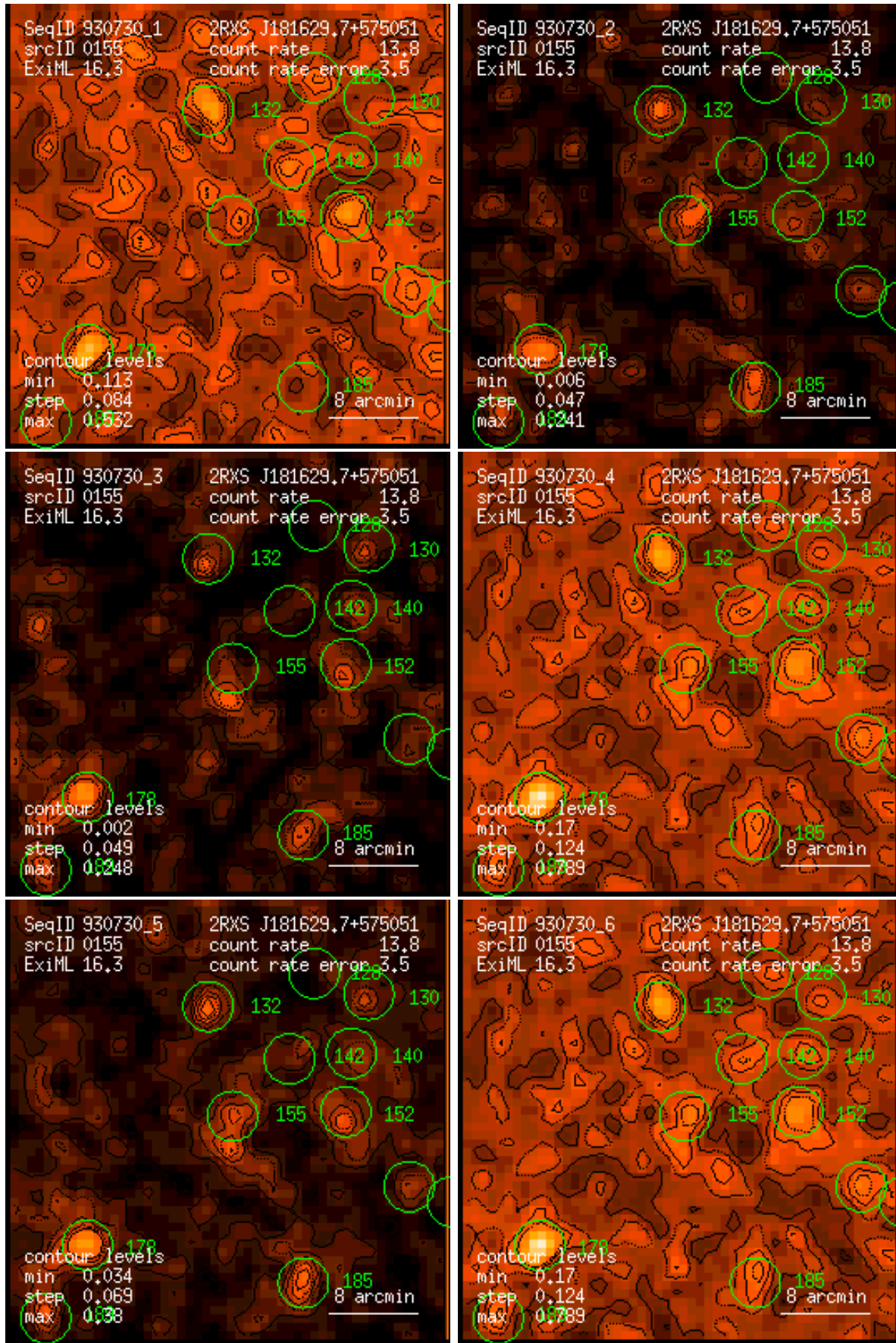
Figure 155: RASS 930730: detection 0155: band rate images, Gaussian filter: (1) PSPC channels 11 – 41, (2) 52 – 90, (3) 91 – 201, (4) 11 – 235, (5) 52 – 201, (6) 11 – 201. Broad band rates in counts/ks. Band rate contour levels in counts/ks/arcmin 2 .
