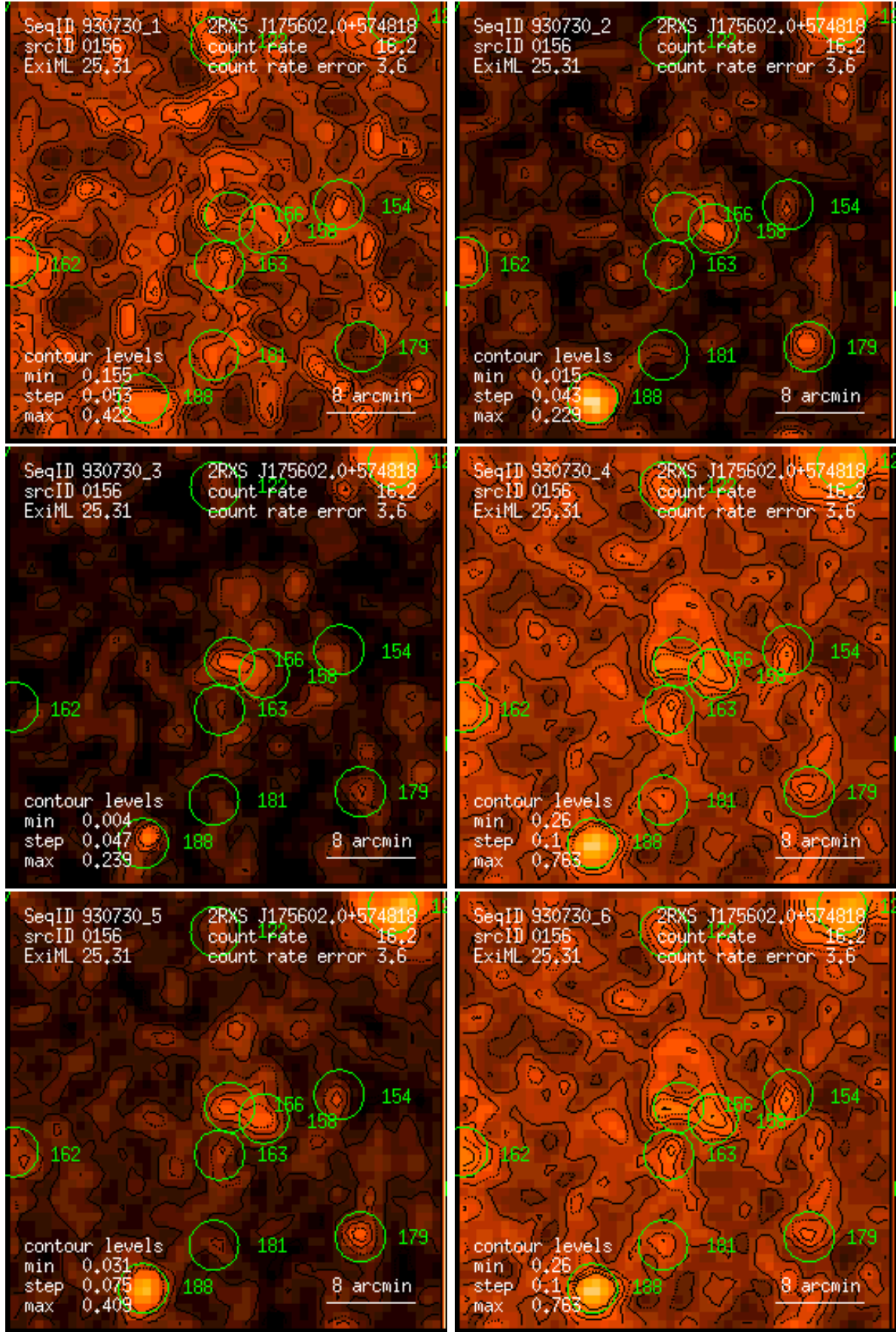
Figure 156: RASS 930730: detection 0156: band rate images, Gaussian filter: (1) PSPC channels 11 – 41, (2) 52 – 90, (3) 91 – 201, (4) 11 – 235, (5) 52 – 201, (6) 11 – 201. Broad band rates in counts/ks. Band rate contour levels in counts/ks/arcmin 2 .
