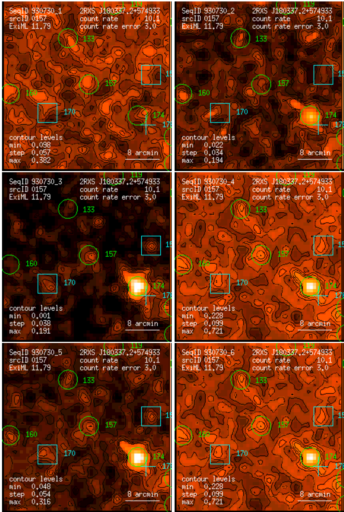
Figure 157: RASS 930730: detection 0157: band rate images, Gaussian filter: (1) PSPC channels 11 – 41, (2) 52 – 90, (3) 91 – 201, (4) 11 – 235, (5) 52 – 201, (6) 11 – 201. Broad band rates in counts/ks. Band rate contour levels in counts/ks/arcmin 2 .
