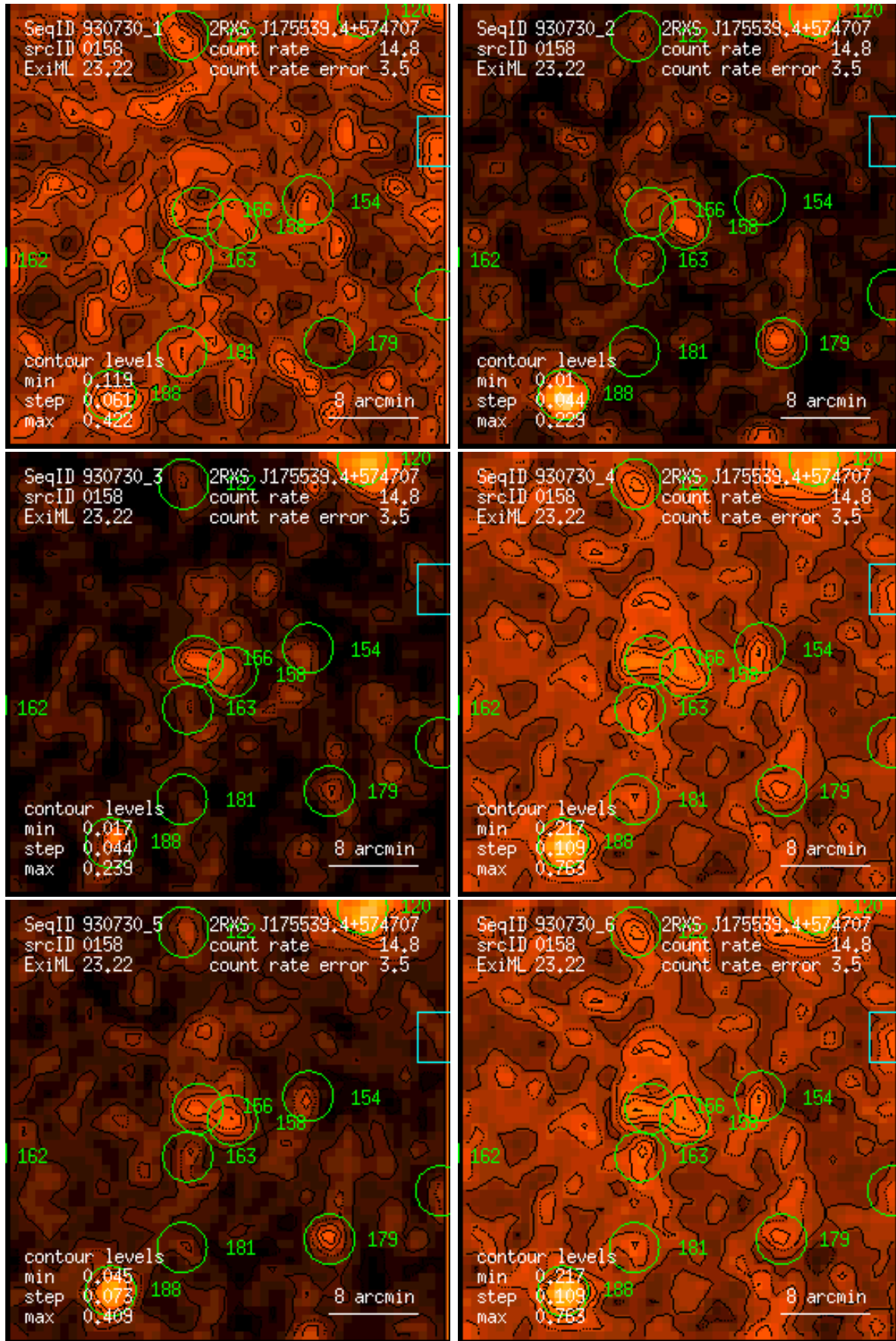
Figure 158: RASS 930730: detection 0158: band rate images, Gaussian filter: (1) PSPC channels 11 – 41, (2) 52 – 90, (3) 91 – 201, (4) 11 – 235, (5) 52 – 201, (6) 11 – 201. Broad band rates in counts/ks. Band rate contour levels in counts/ks/arcmin 2 .
