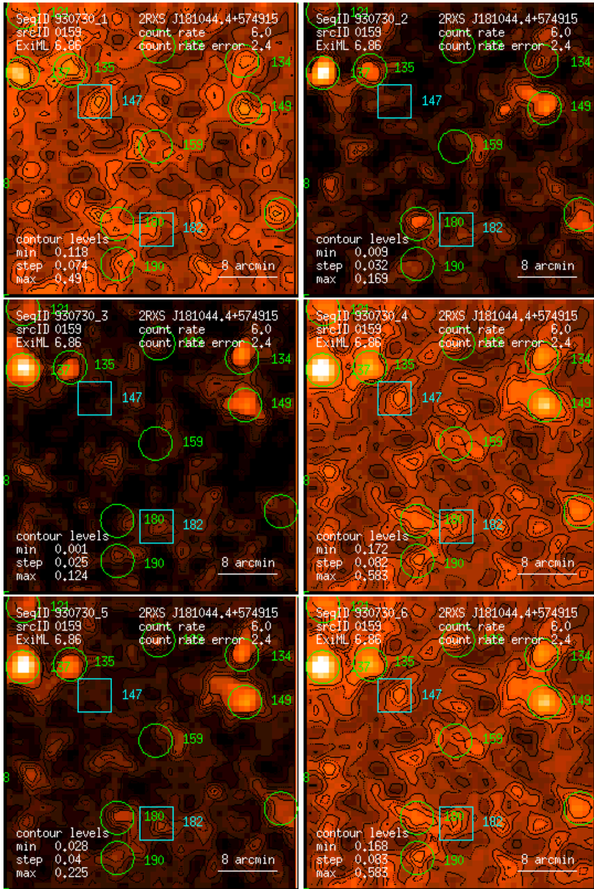
Figure 159: RASS 930730: detection 0159: band rate images, Gaussian filter: (1) PSPC channels 11 – 41, (2) 52 – 90, (3) 91 – 201, (4) 11 – 235, (5) 52 – 201, (6) 11 – 201. Broad band rates in counts/ks. Band rate contour levels in counts/ks/arcmin 2 .
