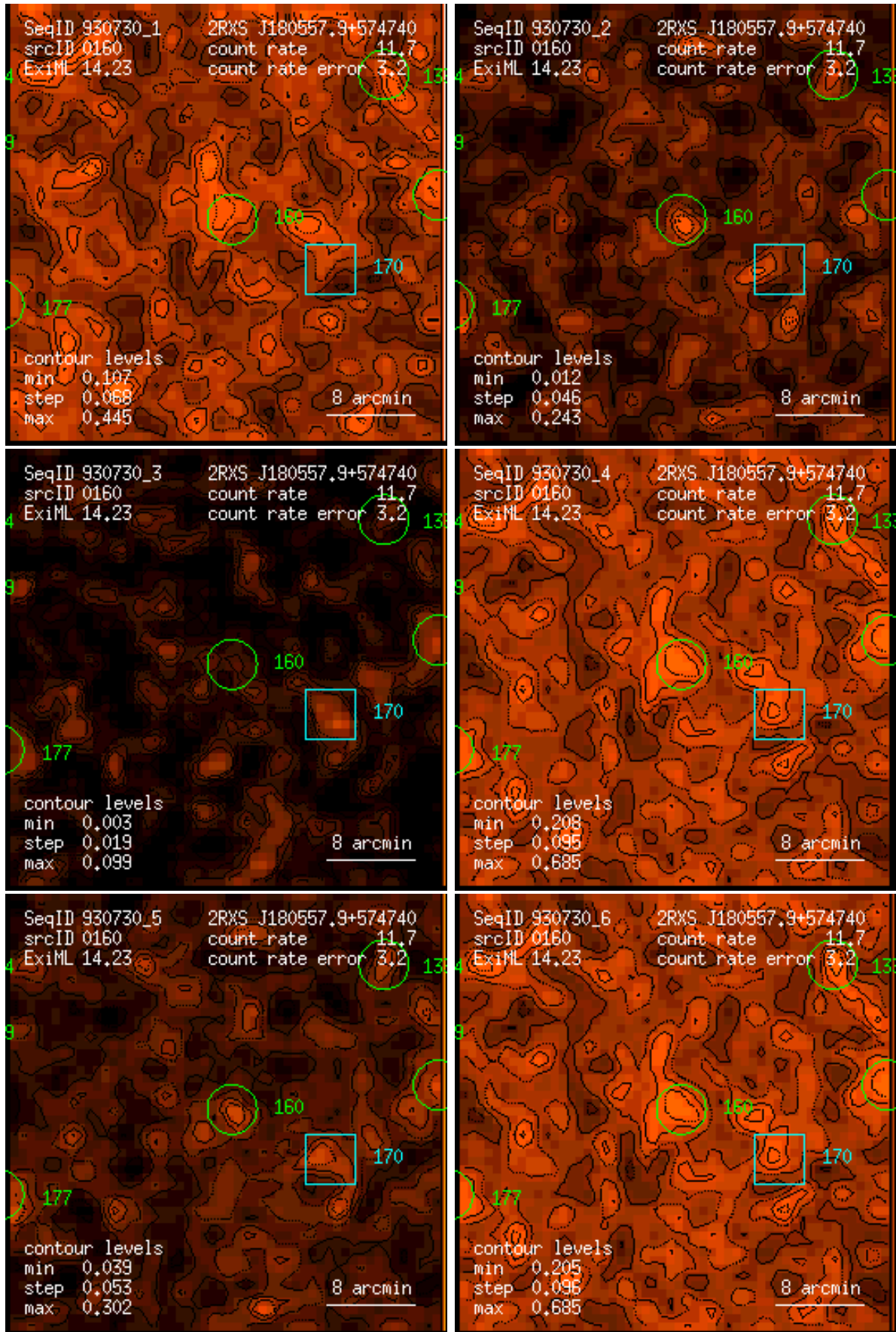
Figure 160: RASS 930730: detection 0160: band rate images, Gaussian filter: (1) PSPPC channels 11 – 41, (2) 52 – 90, (3) 91 – 201, (4) 11 – 235, (5) 52 – 201, (6) 11 – 201. Broad band rates in counts/ks. Band rate contour levels in counts/ks/arcmin 2 .
