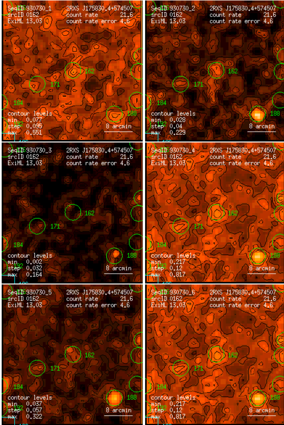
Figure 162: RASS 930730: detection 0162: band rate images, Gaussian filter: (1) PSPC channels 11 – 41, (2) 52 – 90, (3) 91 – 201, (4) 11 – 235, (5) 52 – 201, (6) 11 – 201. Broad band rates in counts/ks. Band rate contour levels in counts/ks/arcmin 2 .
