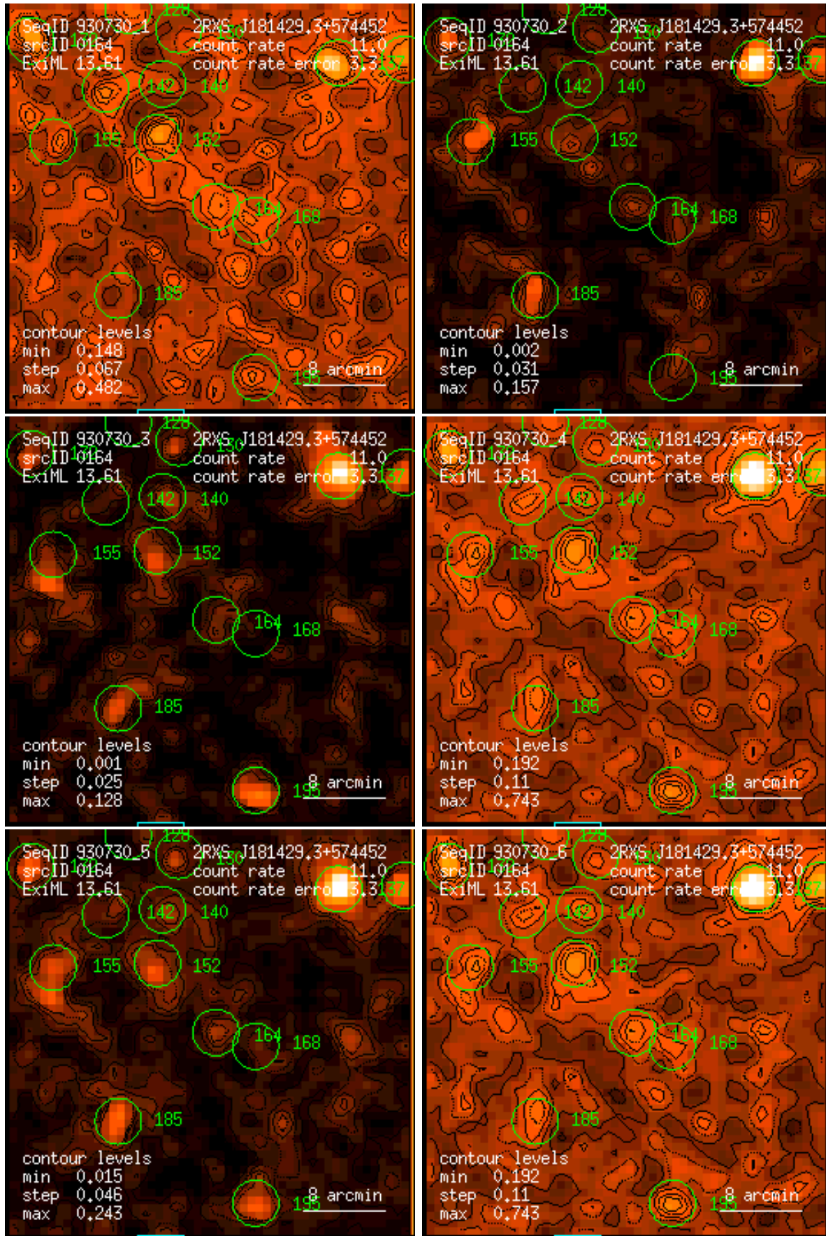
Figure 164: RASS 930730: detection 0164: band rate images, Gaussian filter: (1) PSPC channels 11 – 41, (2) 52 – 90, (3) 91 – 201, (4) 11 – 235, (5) 52 – 201, (6) 11 – 201. Broad band rates in counts/ks. Band rate contour levels in counts/ks/arcmin 2 .
