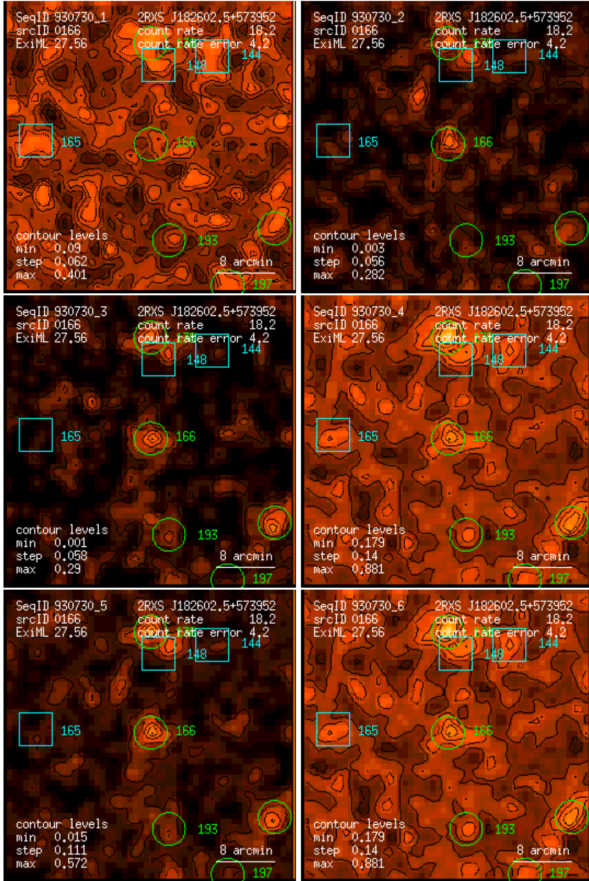
Figure 166: RASS 930730: detection 0166: band rate images, Gaussian filter: (1) PSPC channels 11 – 41, (2) 52 – 90, (3) 91 – 201, (4) 11 – 235, (5) 52 – 201, (6) 11 – 201. Broad band rates in counts/ks. Band rate contour levels in counts/ks/arcmin 2 .
