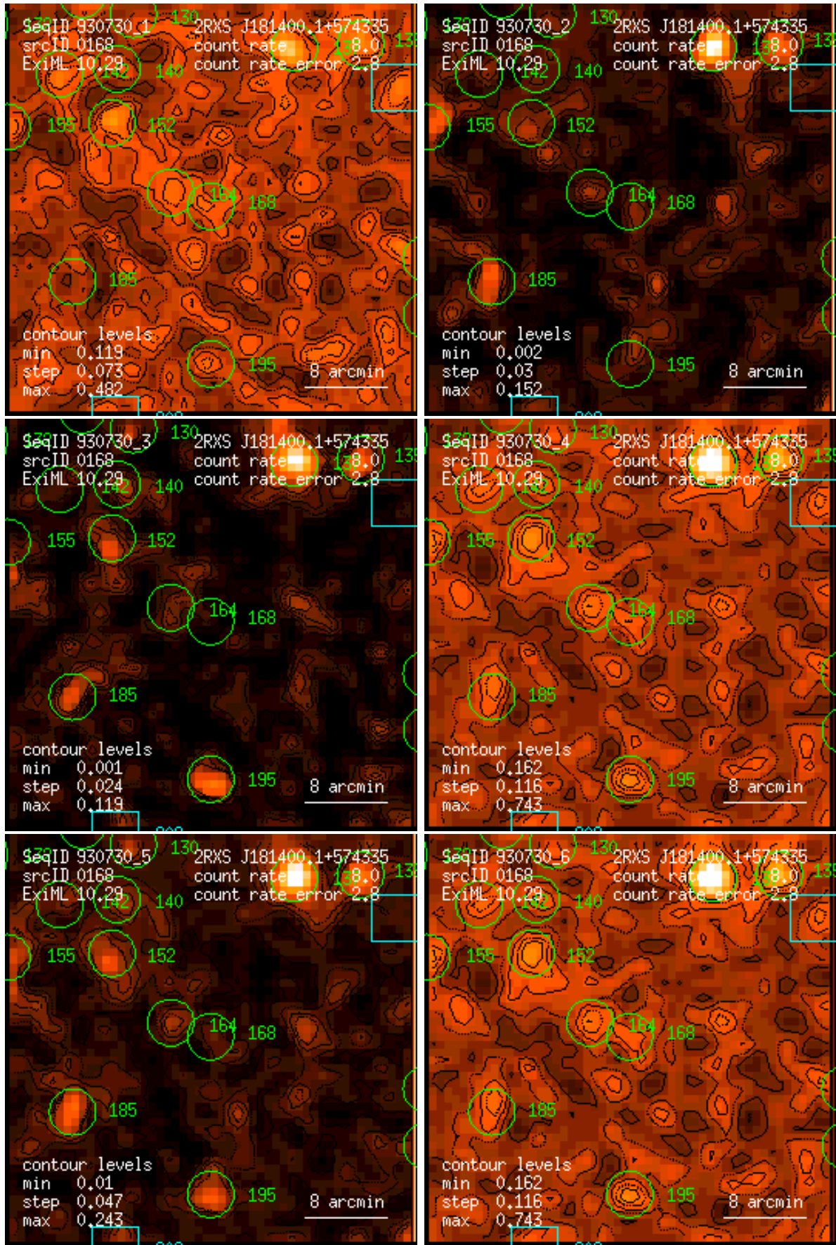
Figure 168: RASS 930730: detection 0168: band rate images, Gaussian filter: (1) PSPC channels 11 – 41, (2) 52 – 90, (3) 91 – 201, (4) 11 – 235, (5) 52 – 201, (6) 11 – 201. Broad band rates in counts/ks. Band rate contour levels in counts/ks/arcmin 2 .
