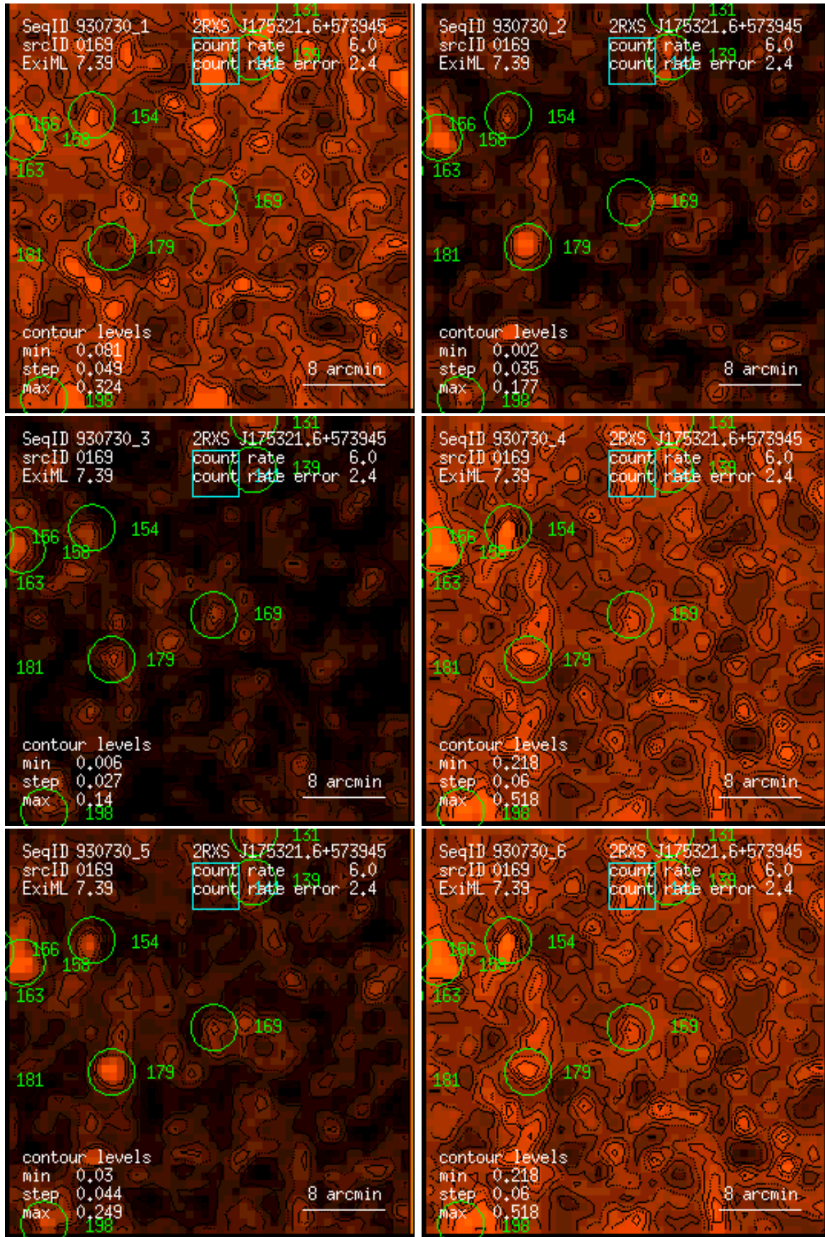
Figure 169: RASS 930730: detection 0169: band rate images, Gaussian filter: (1) PSPC channels 11 – 41, (2) 52 – 90, (3) 91 – 201, (4) 11 – 235, (5) 52 – 201, (6) 11 – 201. Broad band rates in counts/ks. Band rate contour levels in counts/ks/arcmin 2 .
