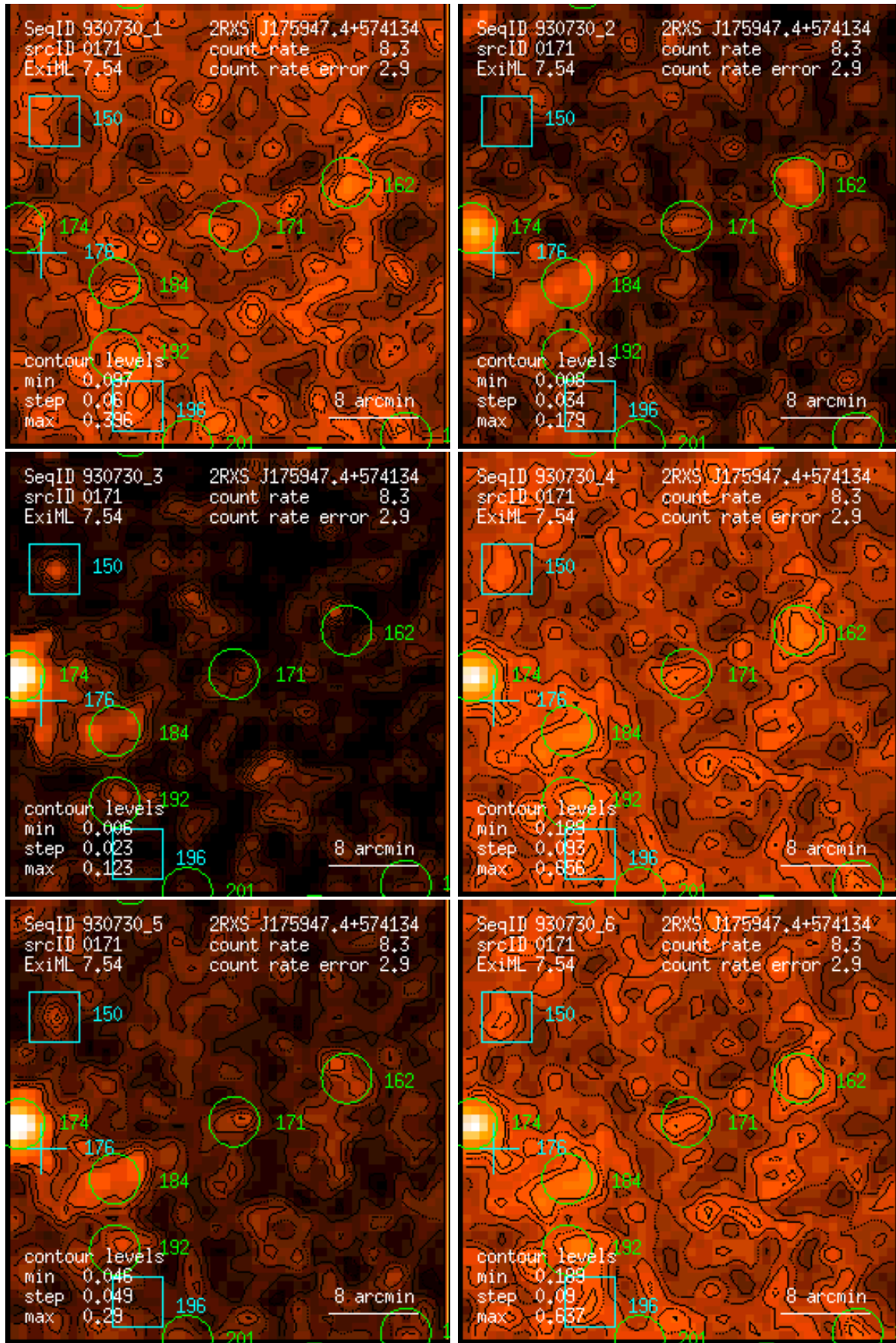
Figure 171: RASS 930730: detection 0171: band rate images, Gaussian filter: (1) PSPC channels 11 – 41, (2) 52 – 90, (3) 91 – 201, (4) 11 – 235, (5) 52 – 201, (6) 11 – 201. Broad band rates in counts/ks. Band rate contour levels in counts/ks/arcmin 2 .
