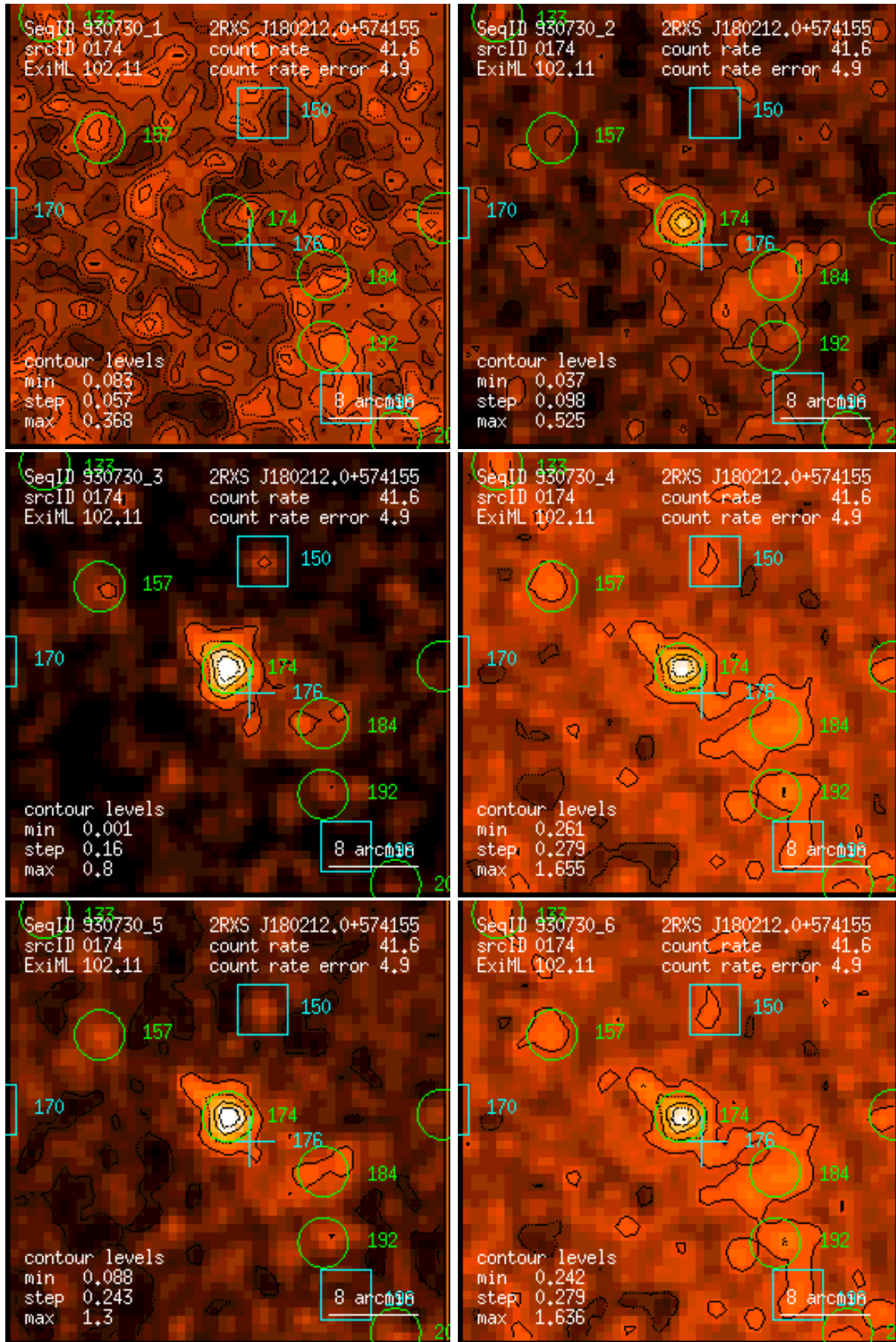
Figure 174: RASS 930730: detection 0174: band rate images, Gaussian filter: (1) PSPC channels 11 – 41, (2) 52 – 90, (3) 91 – 201, (4) 11 – 235, (5) 52 – 201, (6) 11 – 201. Broad band rates in counts/ks. Band rate contour levels in counts/ks/arcmin 2 .
