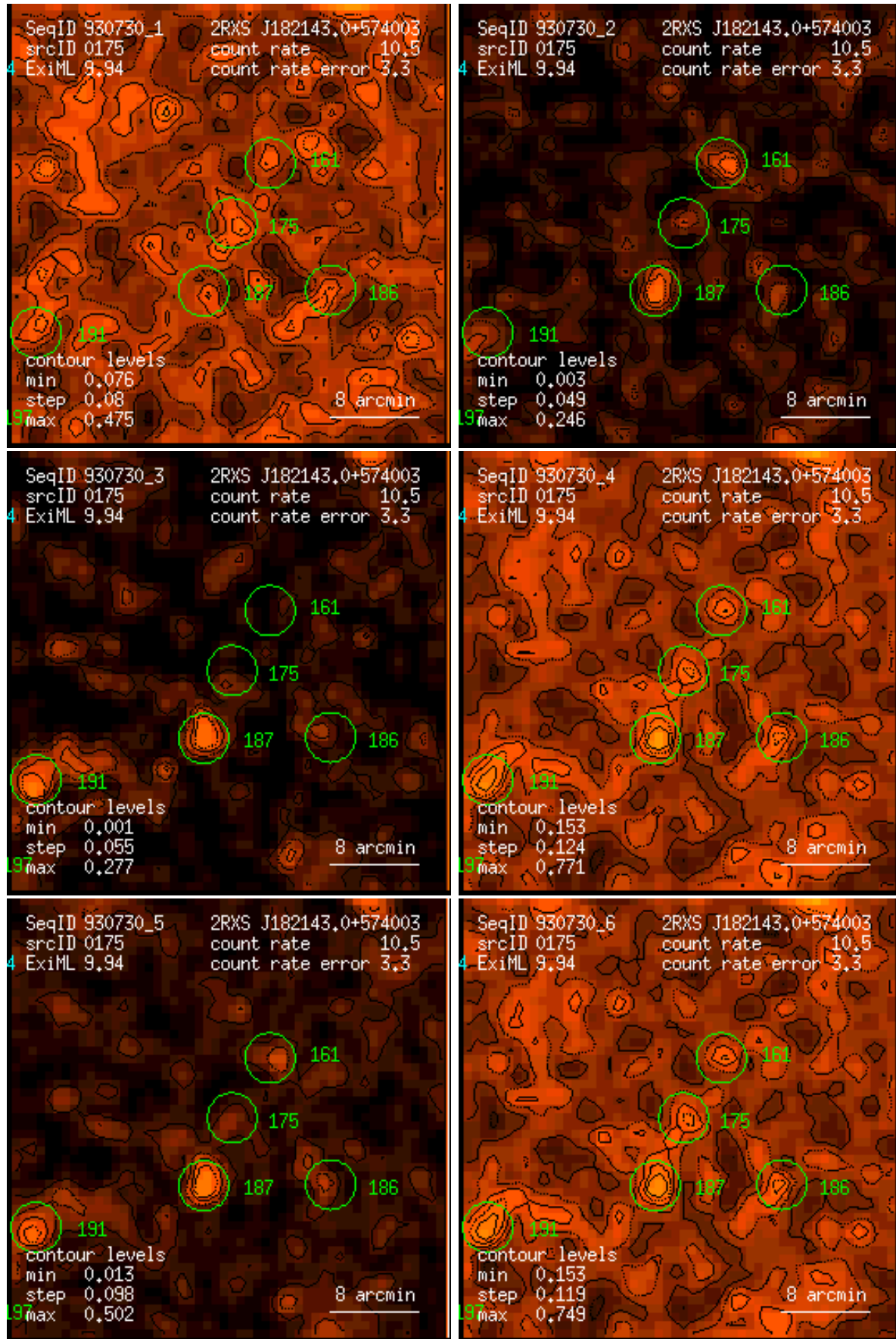
Figure 175: RASS 930730: detection 0175: band rate images, Gaussian filter: (1) PSPC channels 11 – 41, (2) 52 – 90, (3) 91 – 201, (4) 11 – 235, (5) 52 – 201, (6) 11 – 201. Broad band rates in counts/ks. Band rate contour levels in counts/ks/arcmin 2 .
