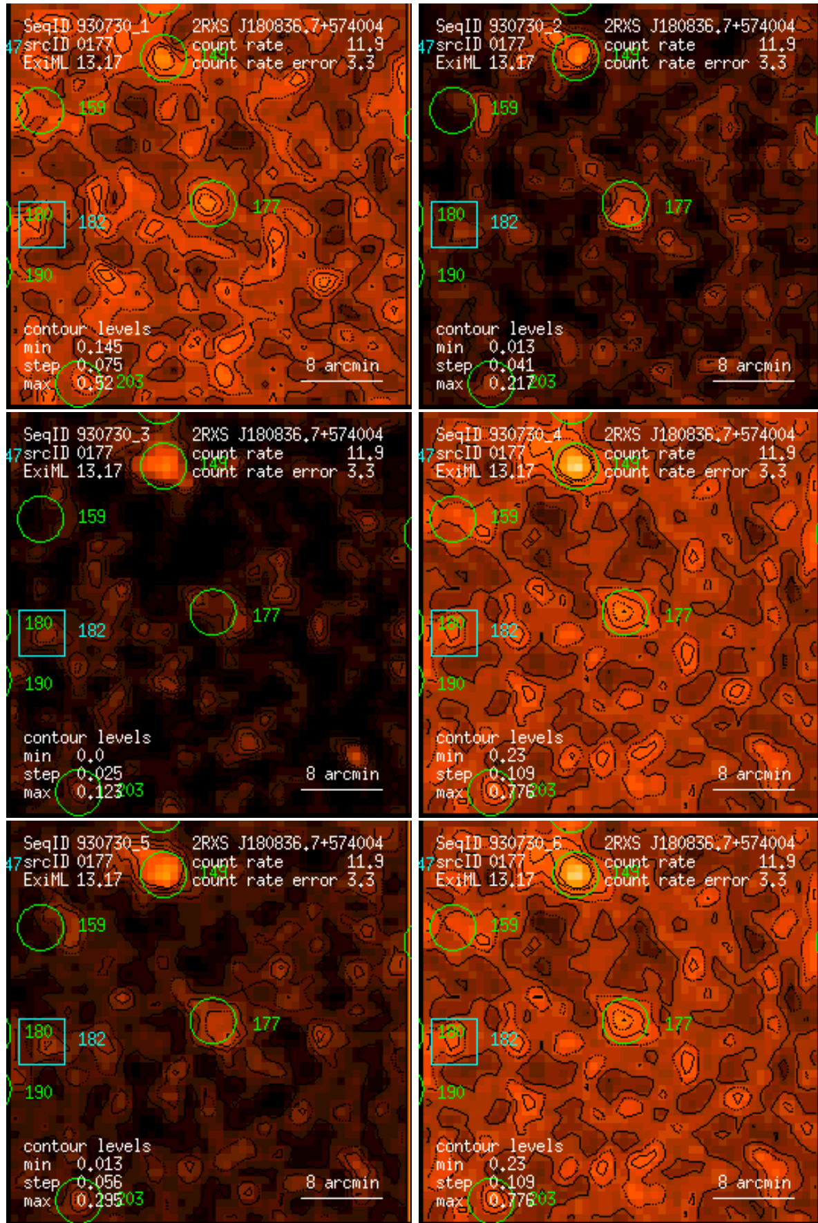
Figure 177: RASS 930730: detection 0177: band rate images, Gaussian filter: (1) PSPC channels 11 – 41, (2) 52 – 90, (3) 91 – 201, (4) 11 – 235, (5) 52 – 201, (6) 11 – 201. Broad band rates in counts/ks. Band rate contour levels in counts/ks/arcmin 2 .
