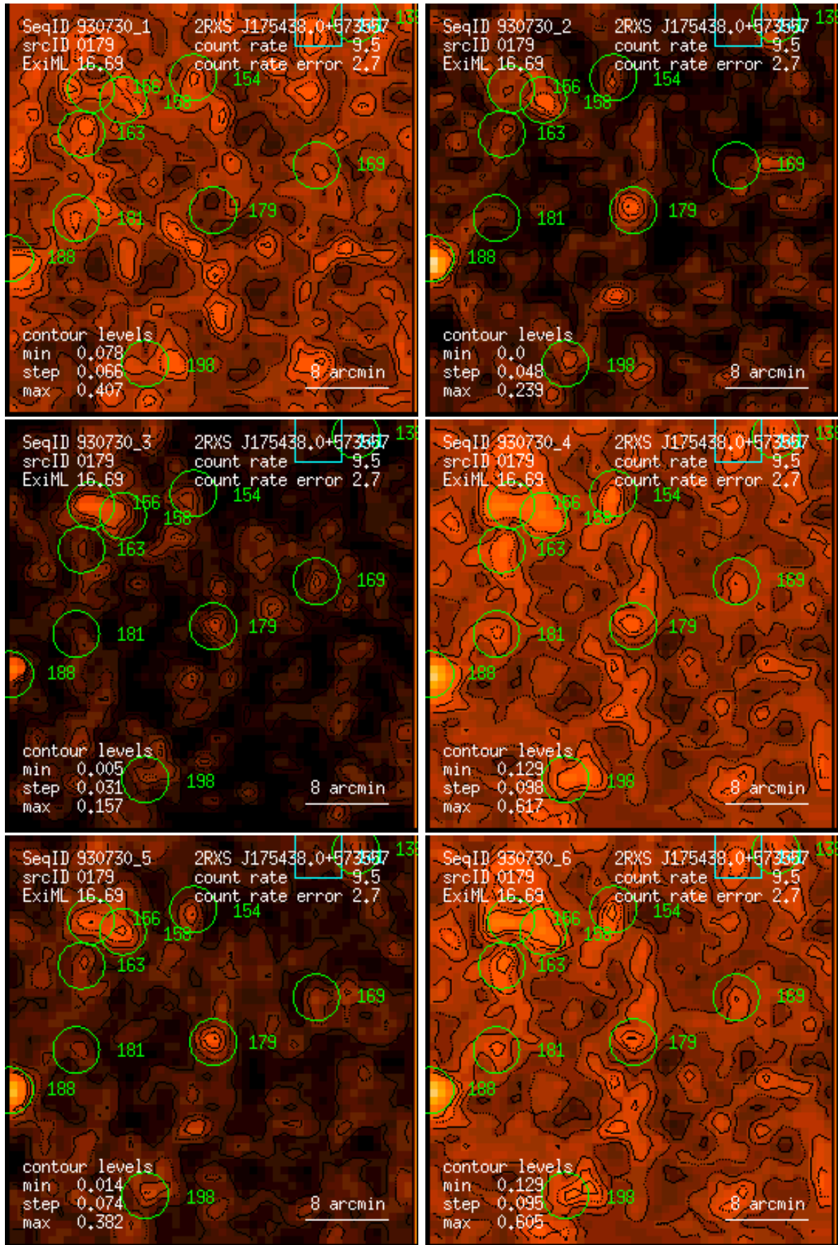
Figure 179: RASS 930730: detection 0179: band rate images, Gaussian filter: (1) PSPC channels 11 – 41, (2) 52 – 90, (3) 91 – 201, (4) 11 – 235, (5) 52 – 201, (6) 11 – 201. Broad band rates in counts/ks. Band rate contour levels in counts/ks/arcmin 2 .
