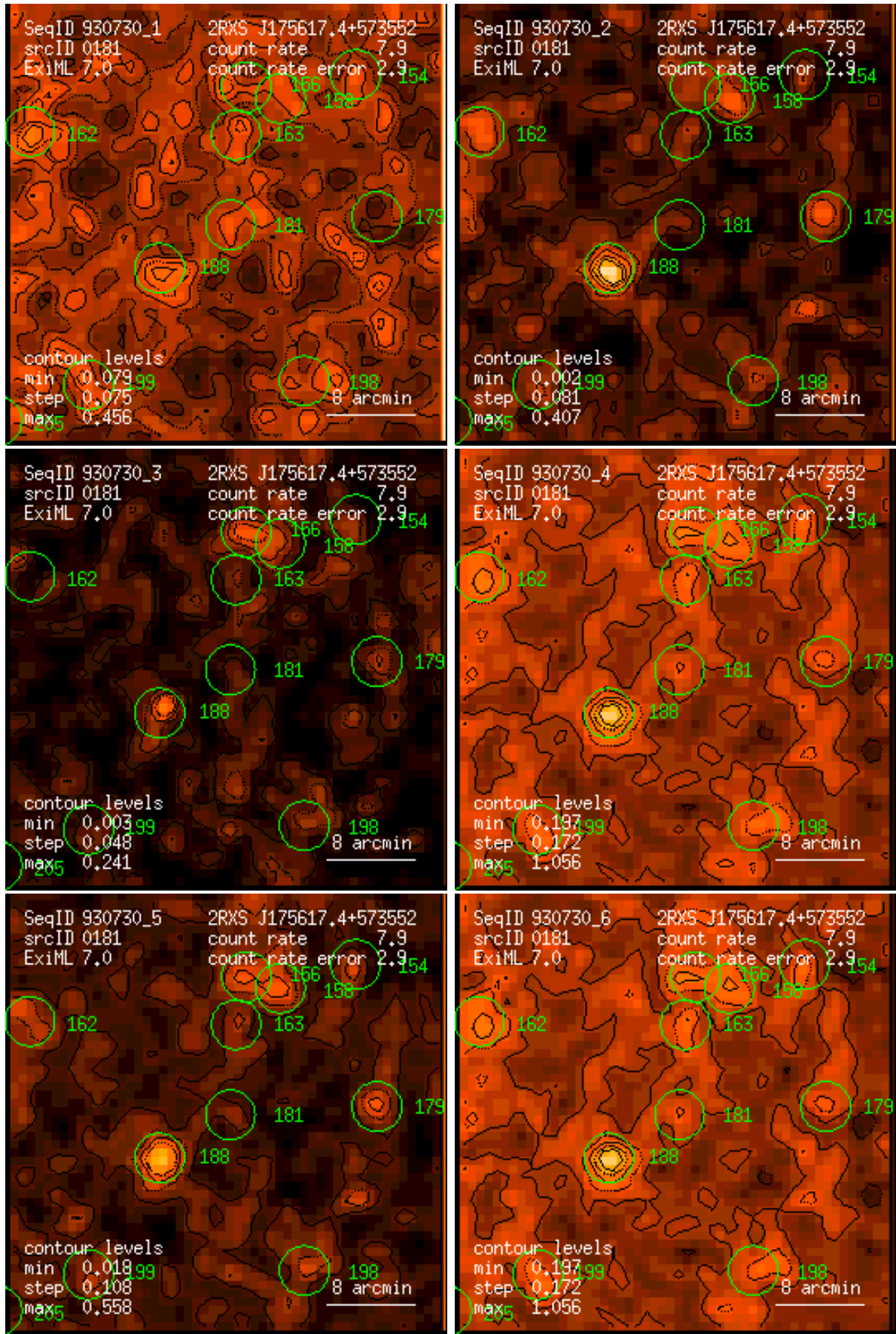
Figure 181: RASS 930730: detection 0181: band rate images, Gaussian filter: (1) PSPC channels 11 – 41, (2) 52 – 90, (3) 91 – 201, (4) 11 – 235, (5) 52 – 201, (6) 11 – 201. Broad band rates in counts/ks. Band rate contour levels in counts/ks/arcmin 2 .
