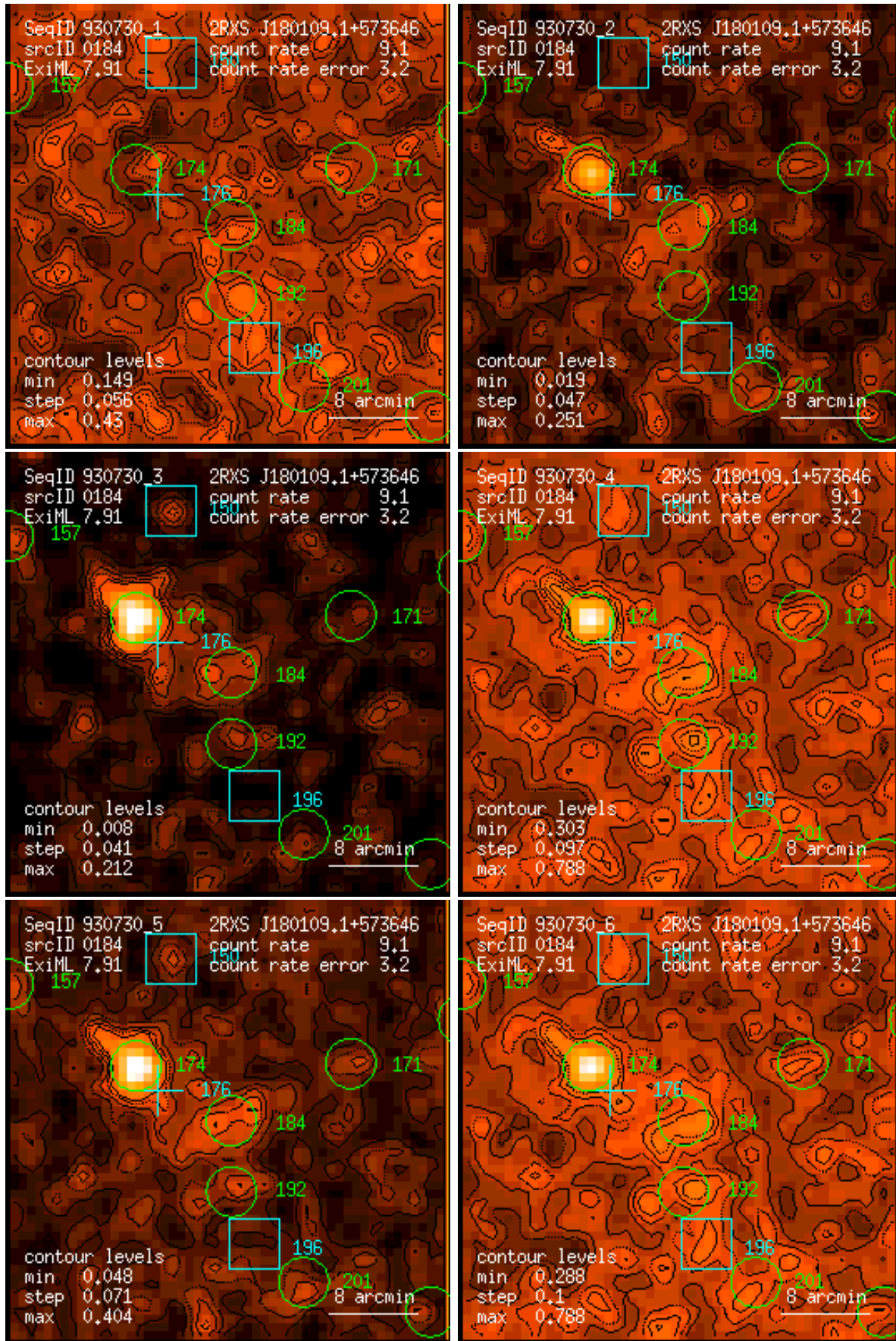
Figure 184: RASS 930730: detection 0184: band rate images, Gaussian filter: (1) PSPC channels 11 – 41, (2) 52 – 90, (3) 91 – 201, (4) 11 – 235, (5) 52 – 201, (6) 11 – 201. Broad band rates in counts/ks. Band rate contour levels in counts/ks/arcmin 2 .
