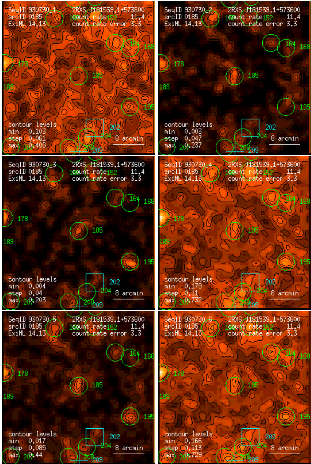
Figure 185: RASS 930730: detection 0185: band rate images, Gaussian filter: (1) PSPC channels 11 – 41, (2) 52 – 90, (3) 91 – 201, (4) 11 – 235, (5) 52 – 201, (6) 11 – 201. Broad band rates in counts/ks. Band rate contour levels in counts/ks/arcmin 2 .
