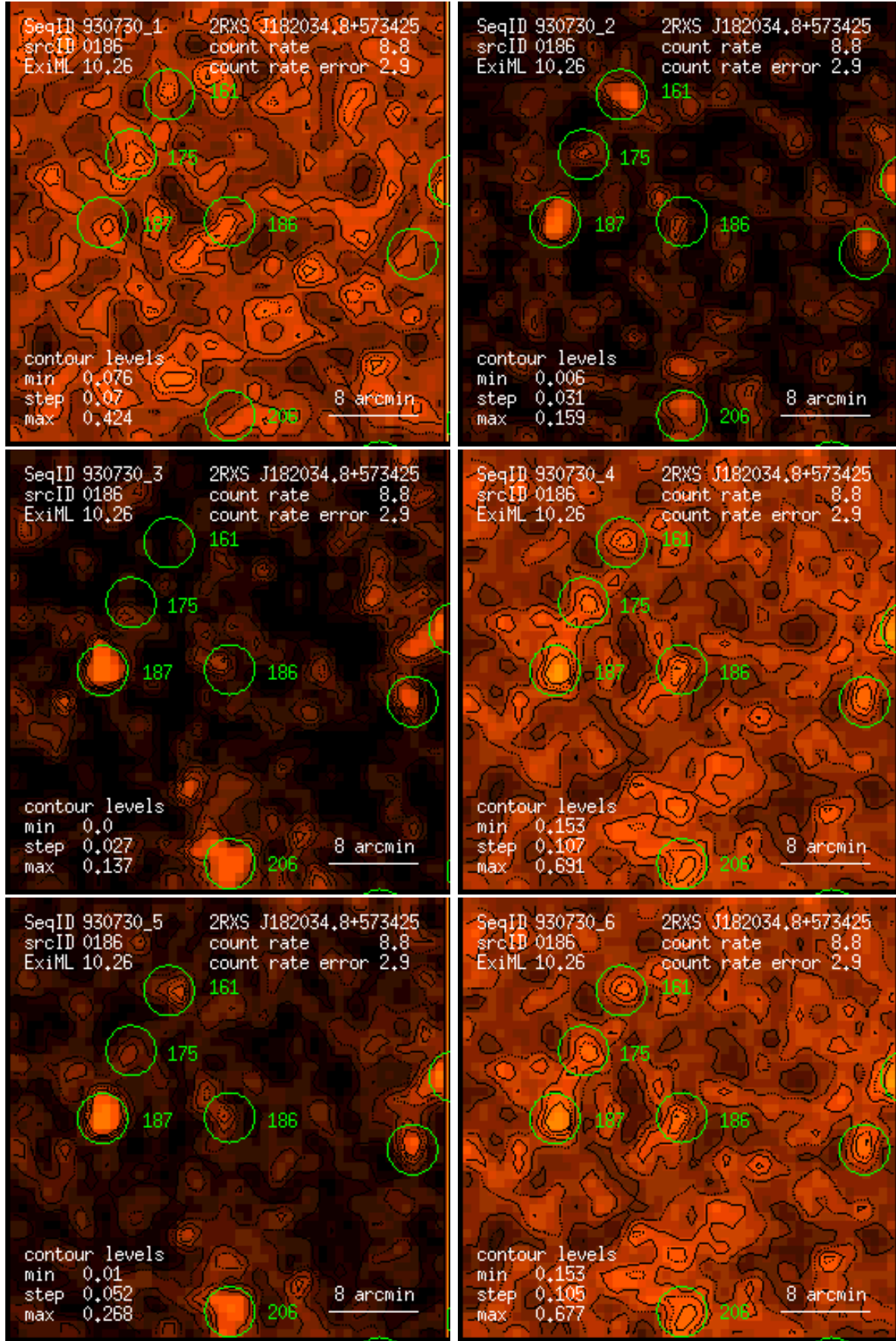
Figure 186: RASS 930730: detection 0186: band rate images, Gaussian filter: (1) PSPC channels 11 – 41, (2) 52 – 90, (3) 91 – 201, (4) 11 – 235, (5) 52 – 201, (6) 11 – 201. Broad band rates in counts/ks. Band rate contour levels in counts/ks/arcmin 2 .
